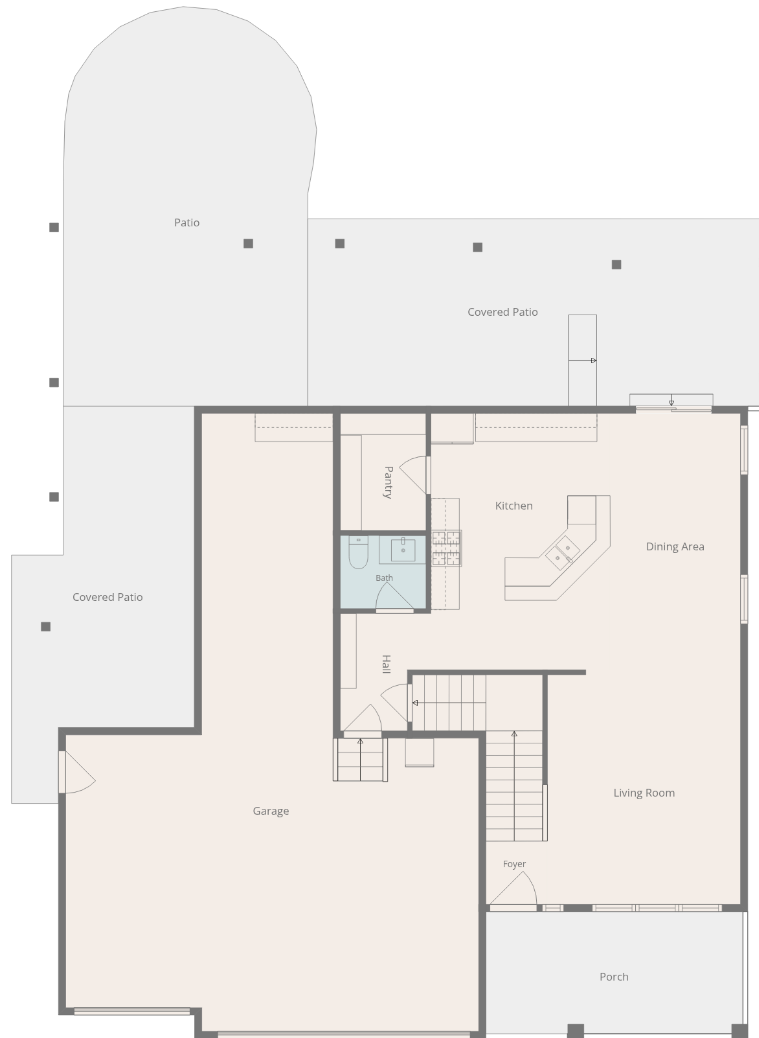
1st Floor
