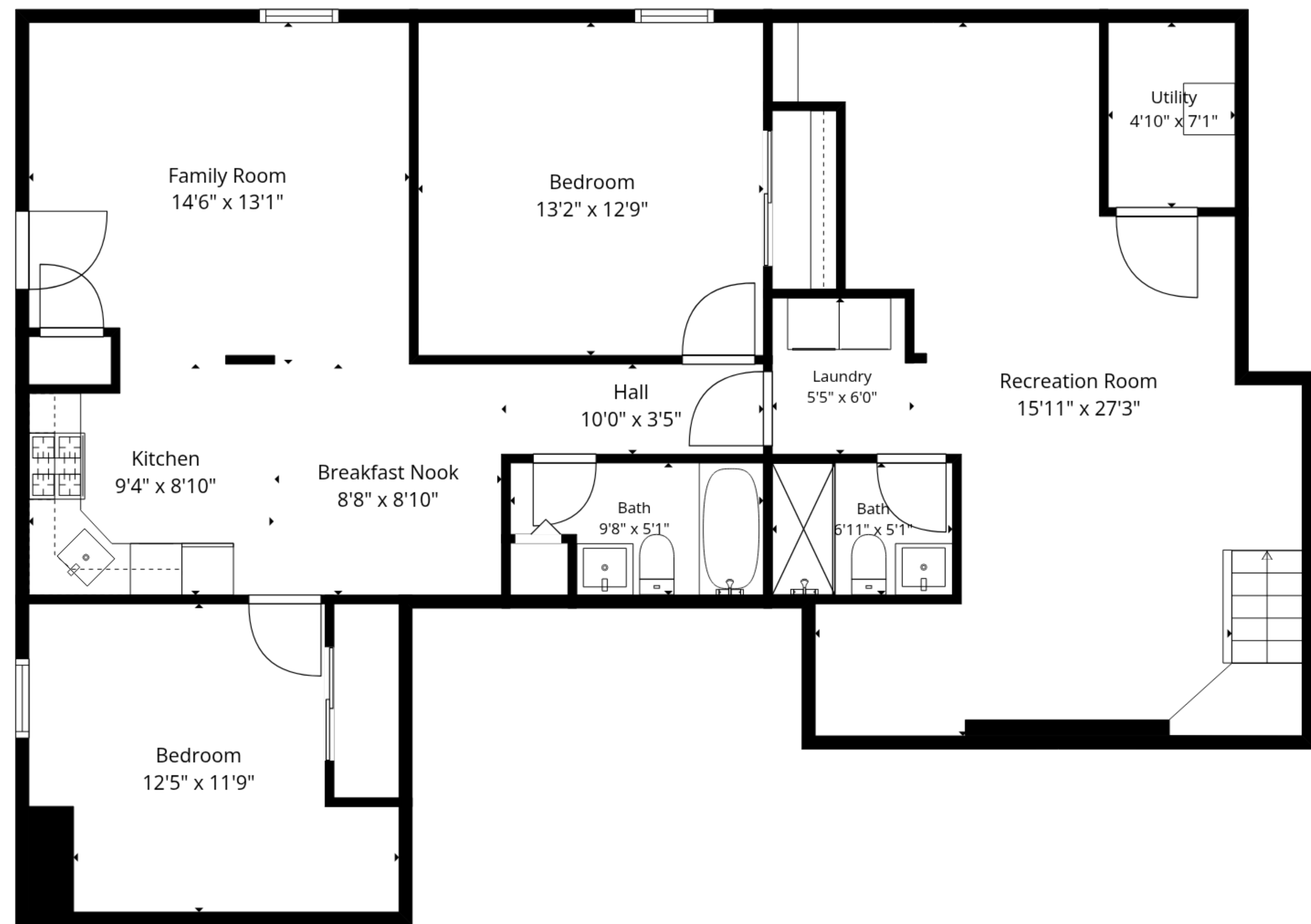
1st Floor
