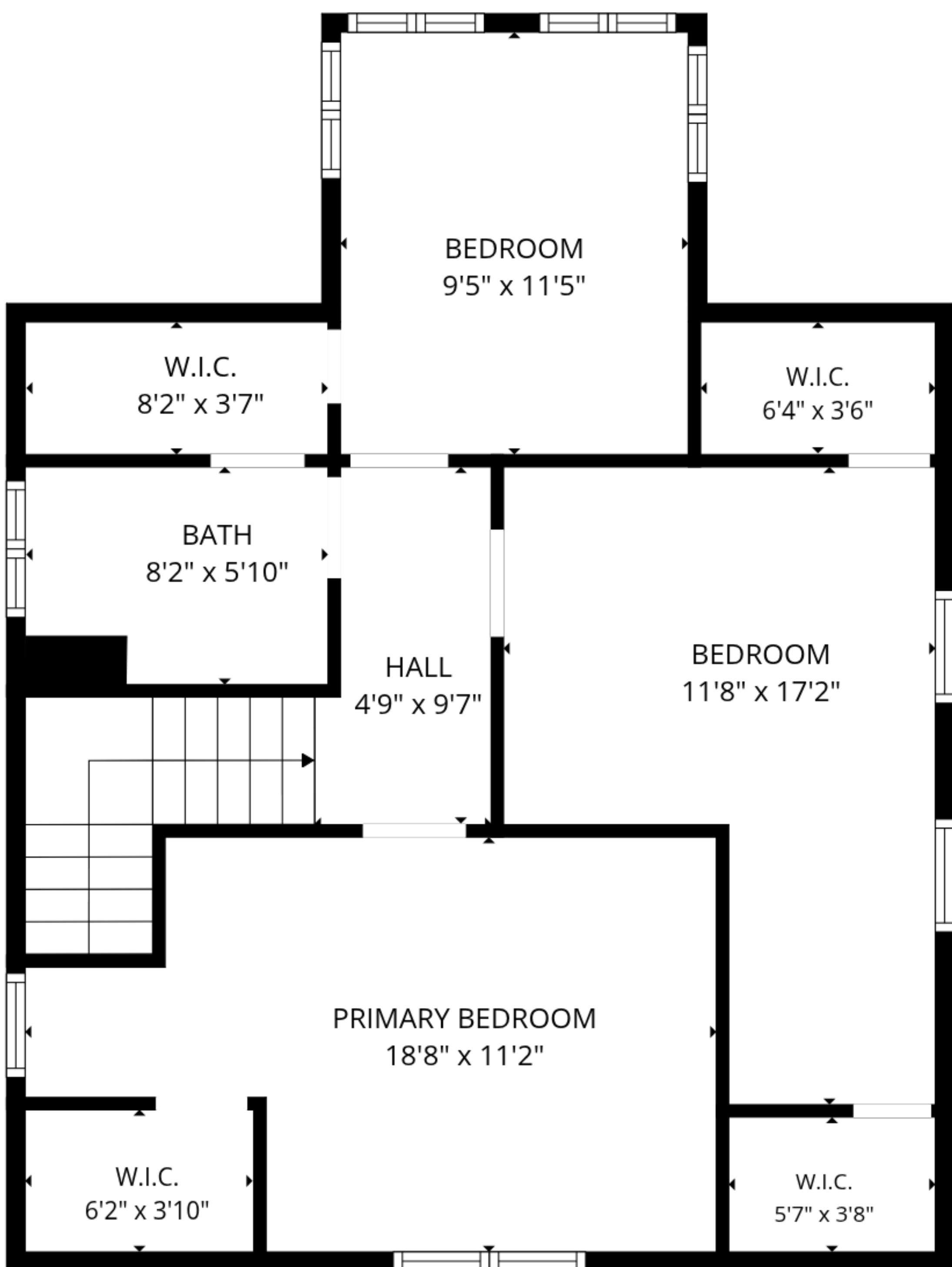
2nd floor
