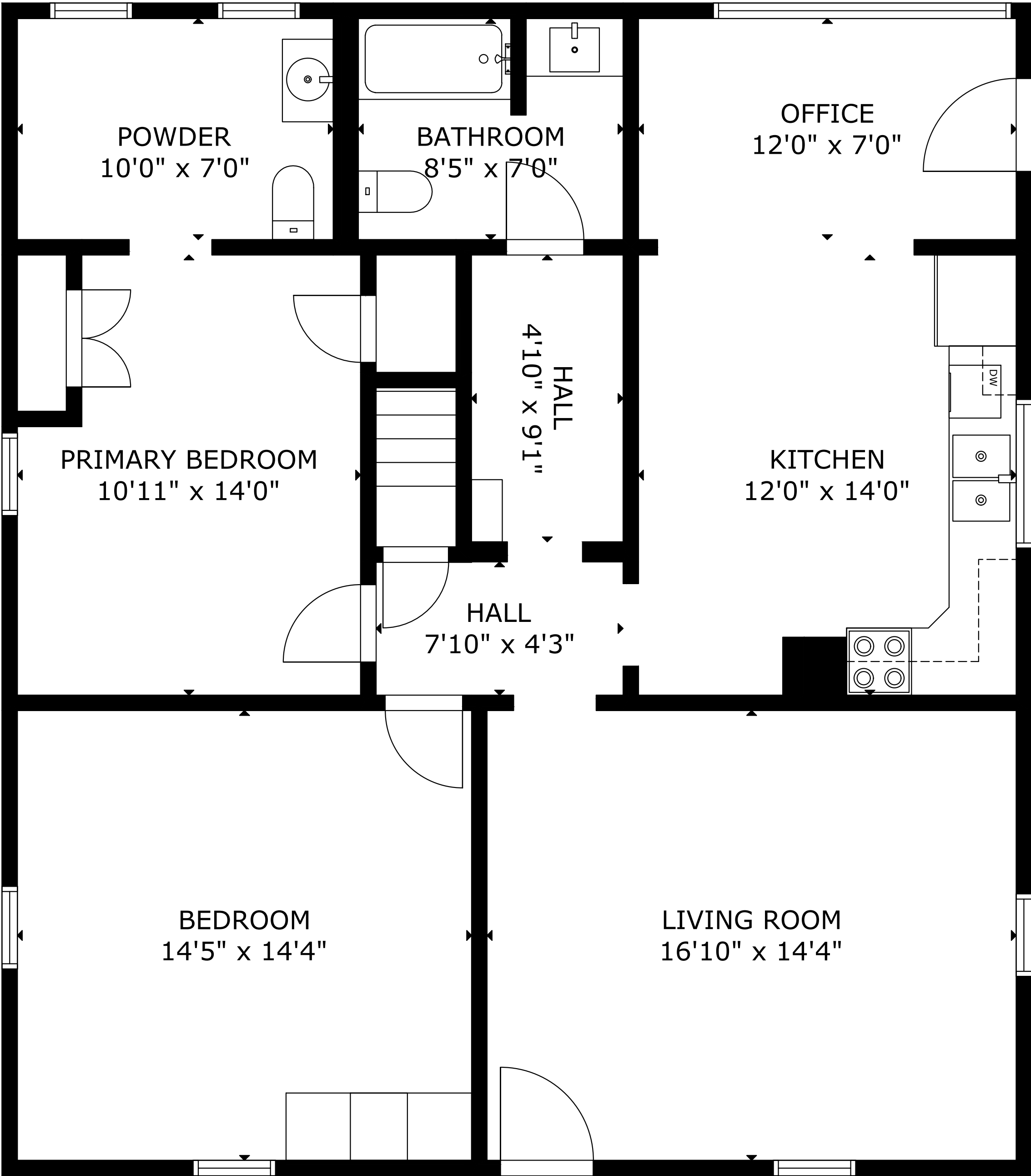
MAIN FLOOR
