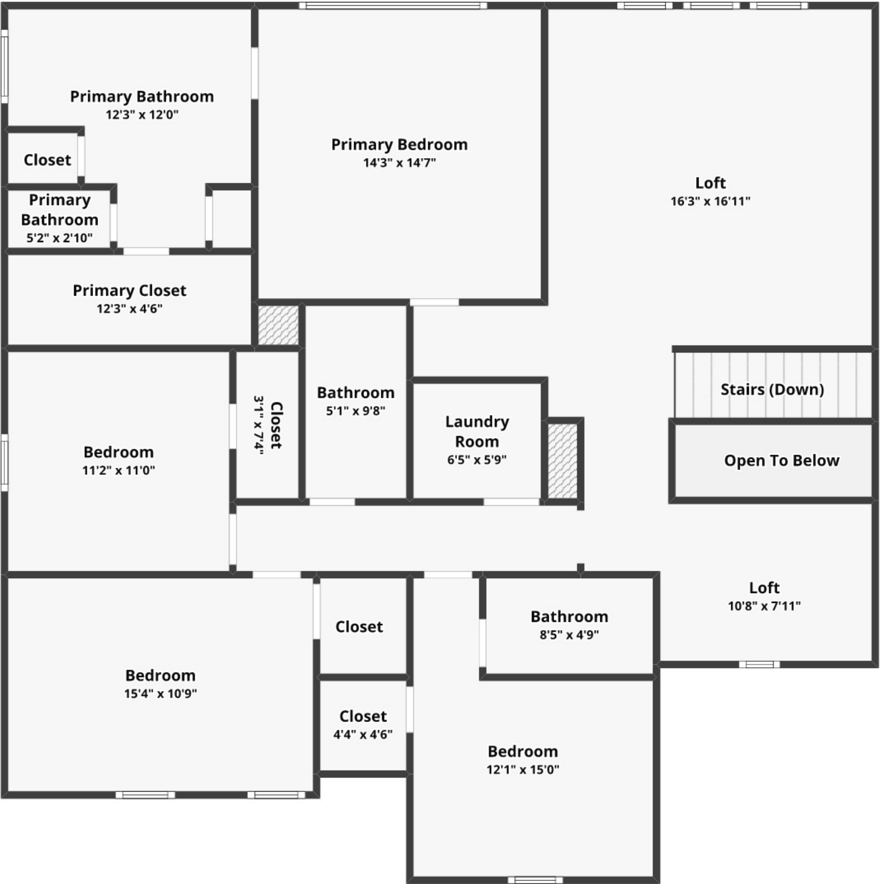
FLOOR 2
