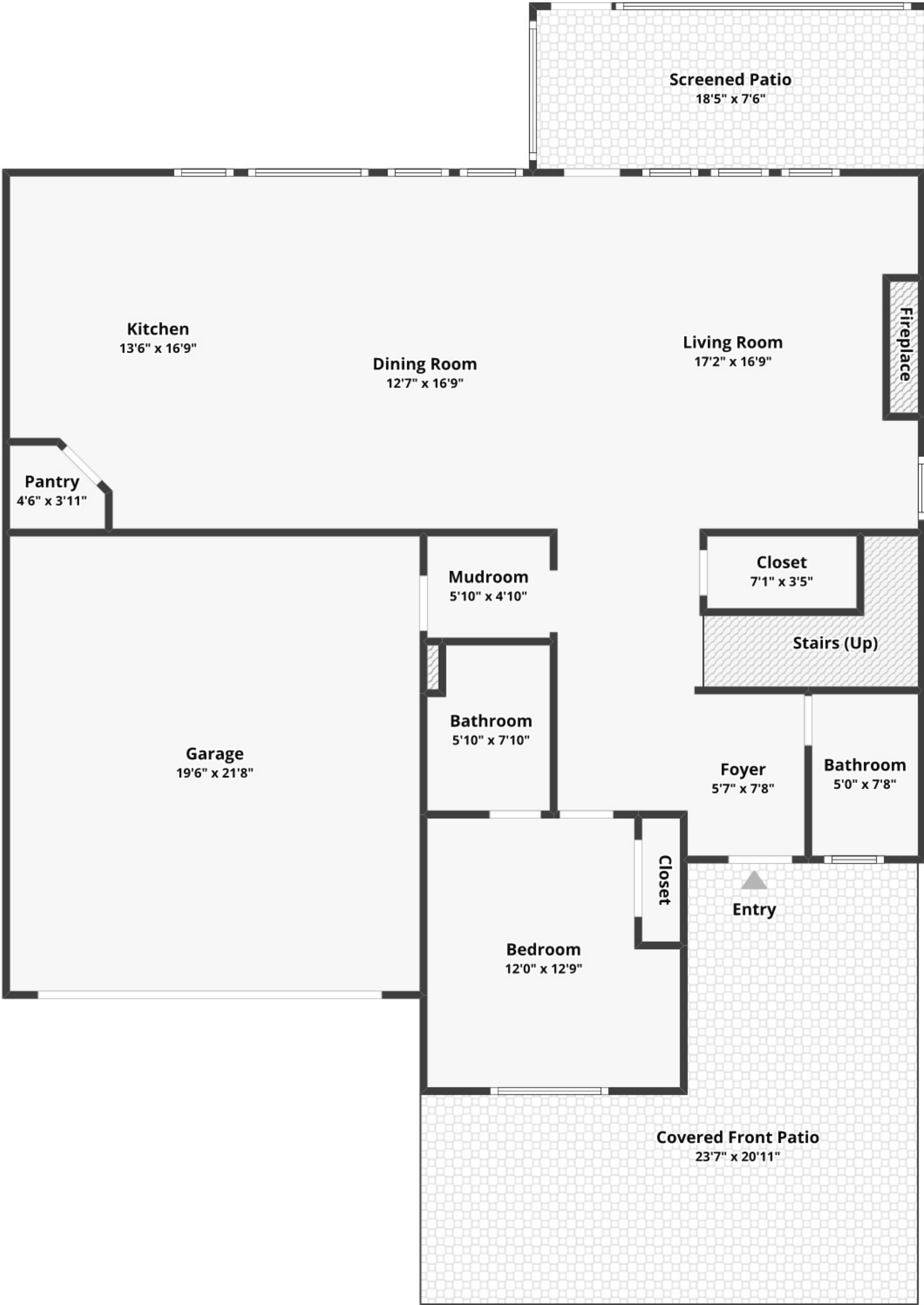
FLOOR 1
