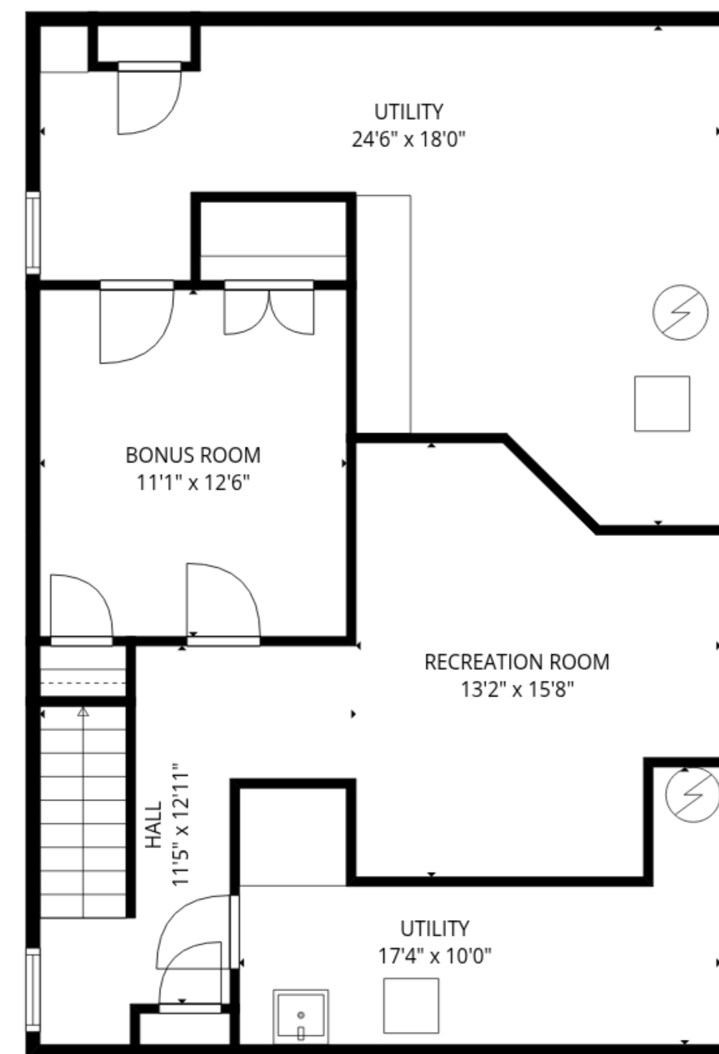
Basement
