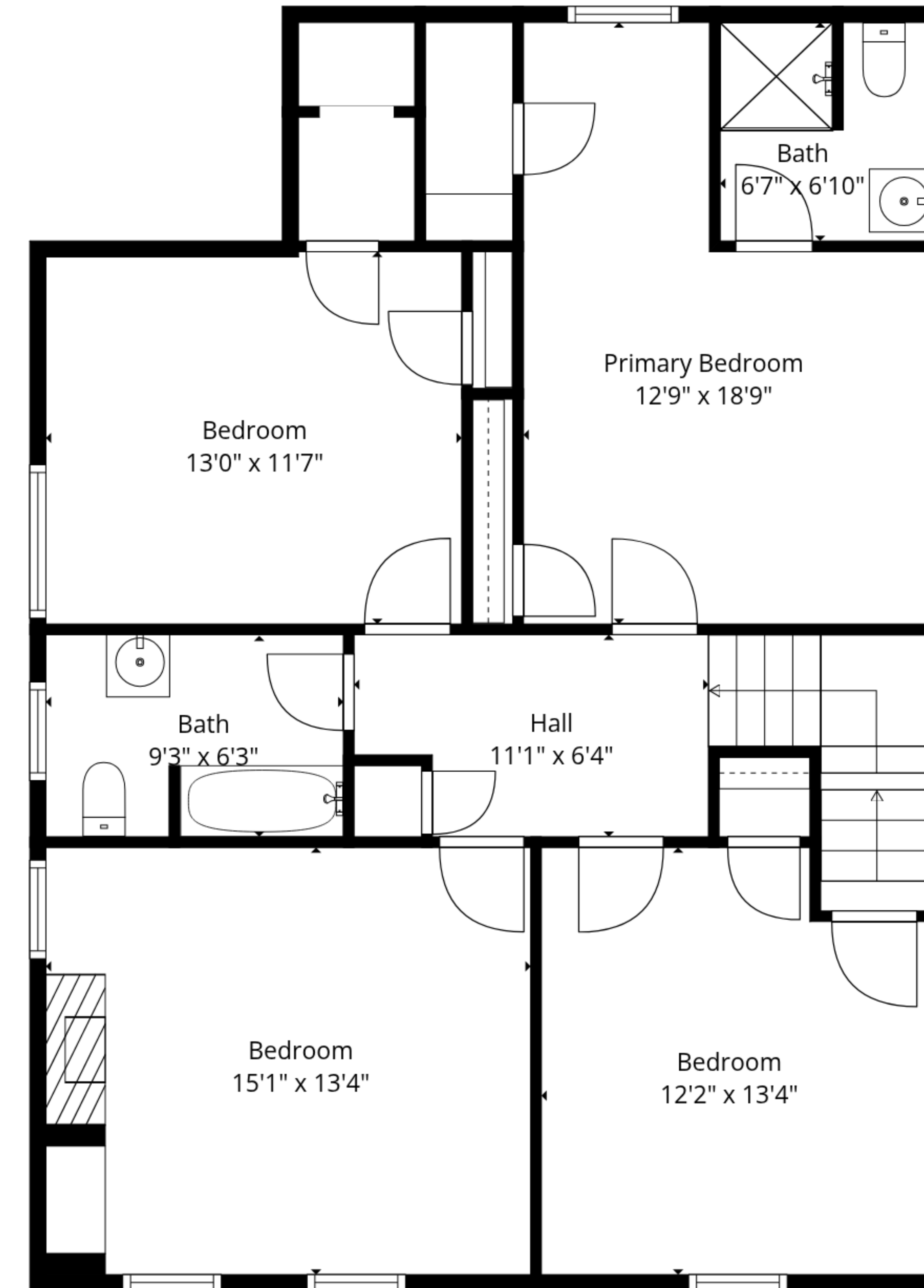
2nd Floor
