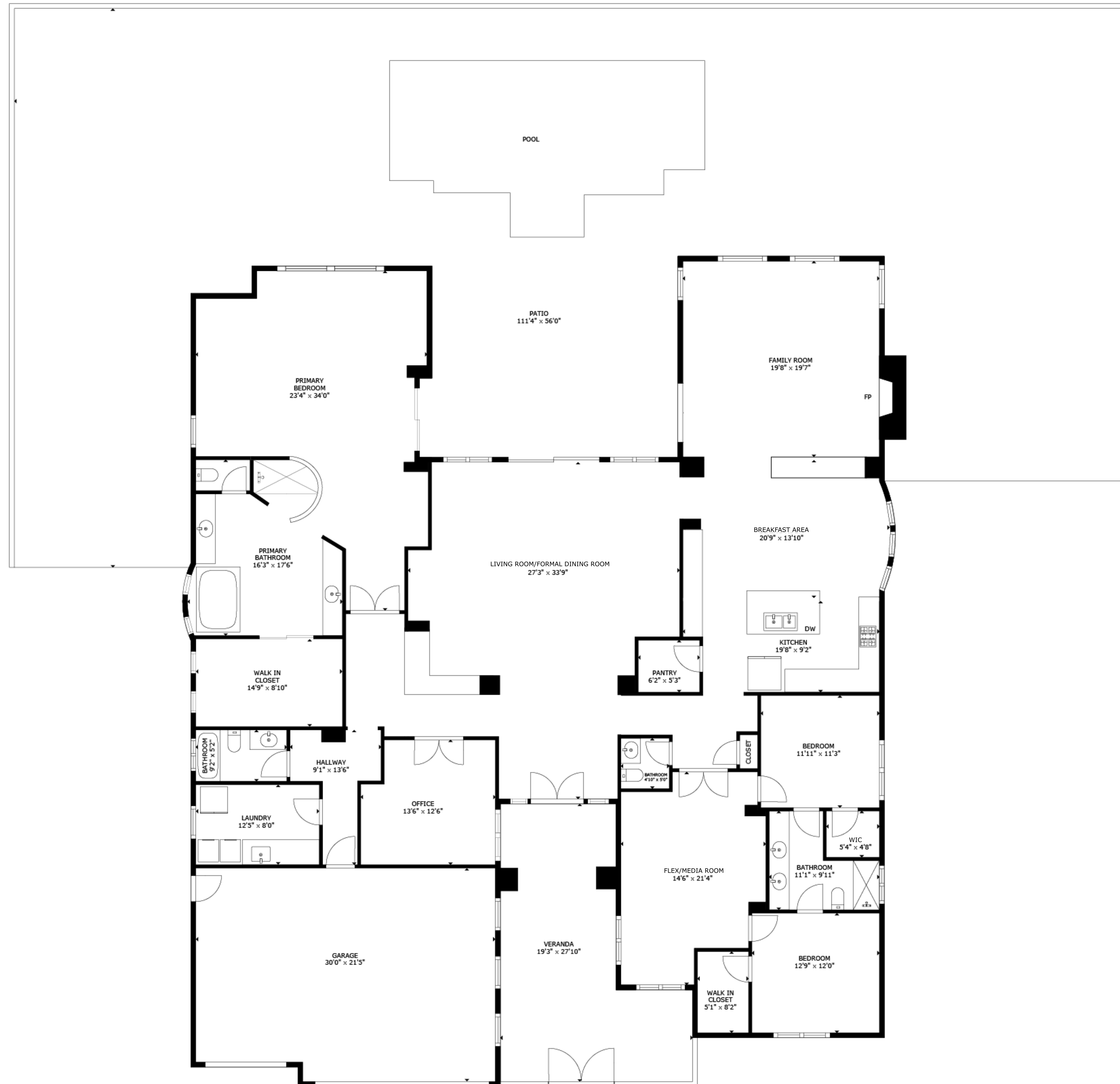
FLOOR PLAN
