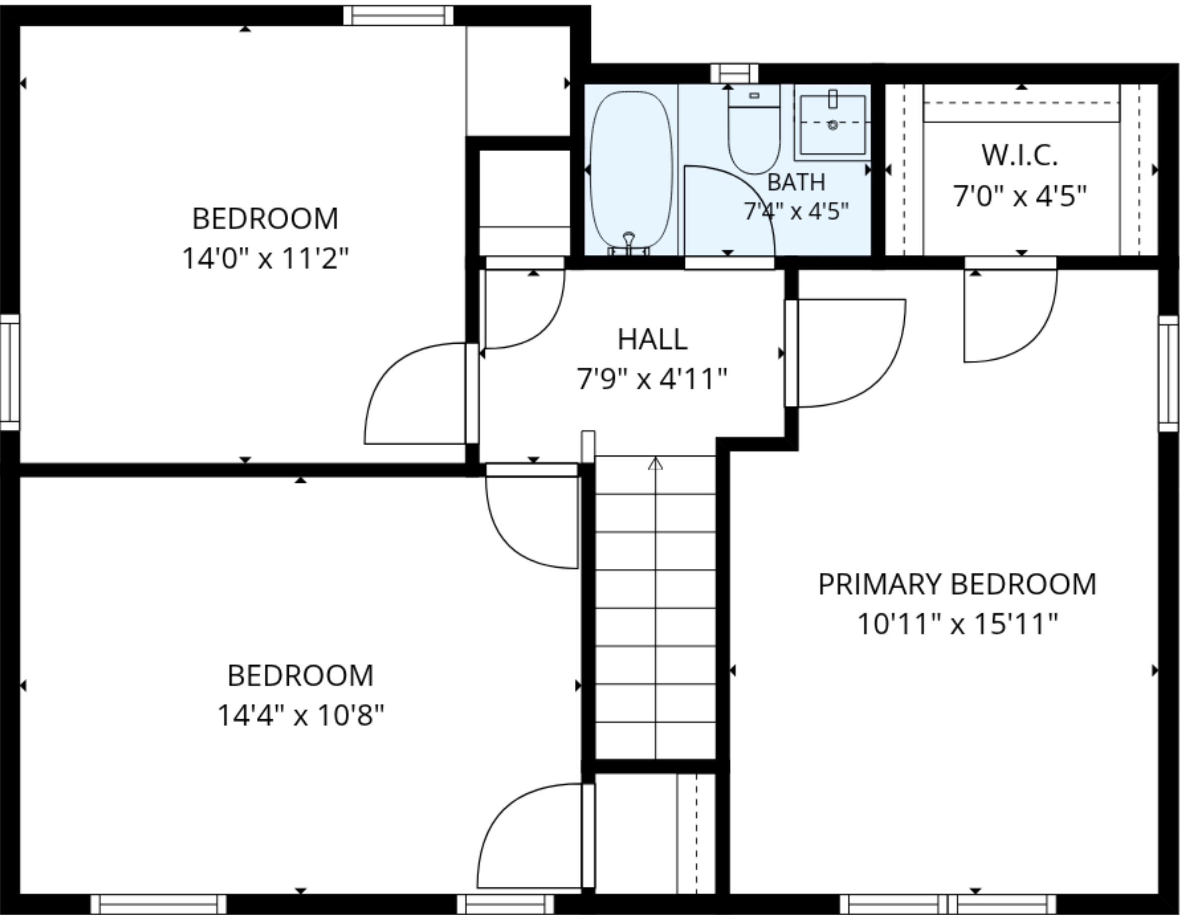
2nd floor
