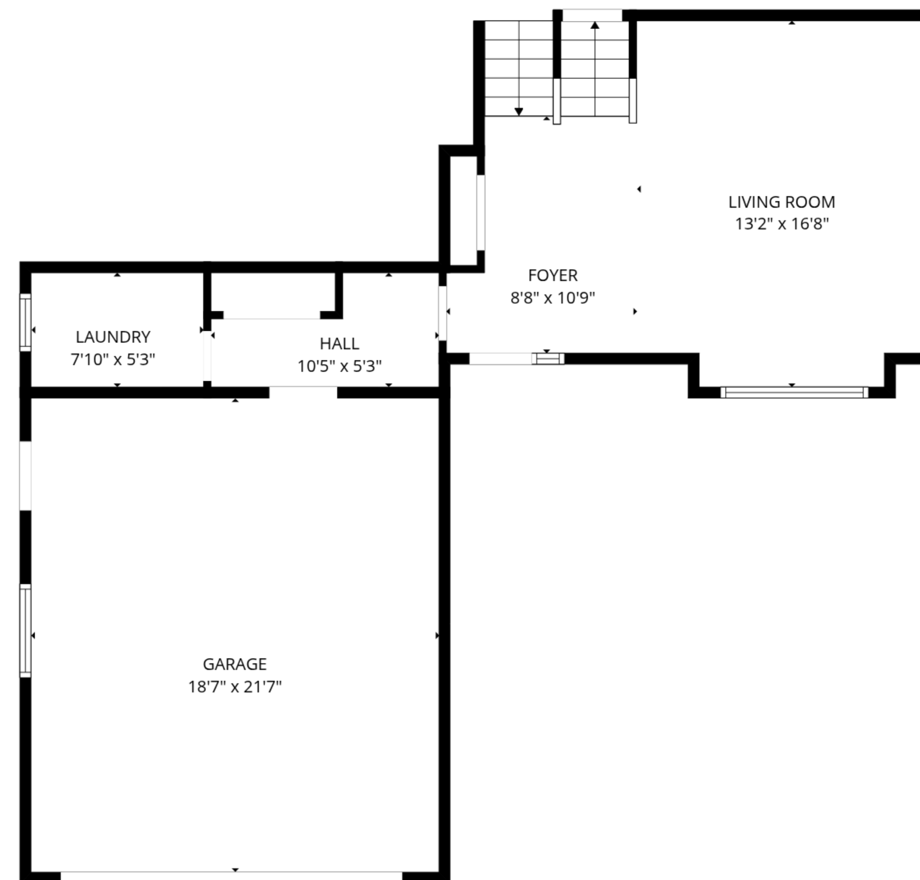
1st floor
