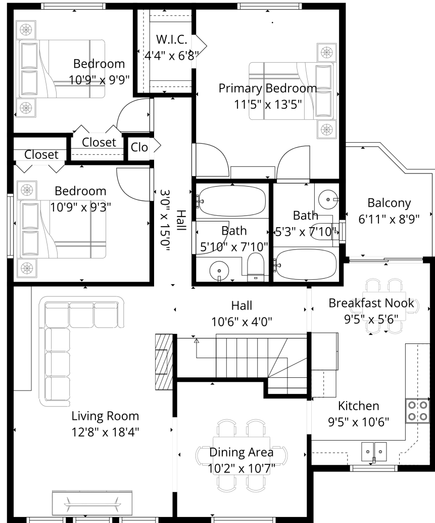
UPPER FLOOR 1,235 SQ.FT. CEILING HEIGHT 8'
