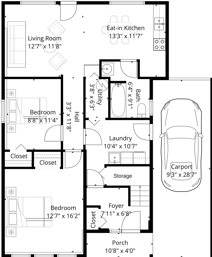
LOWER FLOOR 996 SQ.FT. CEILING HEIGHT 8'
