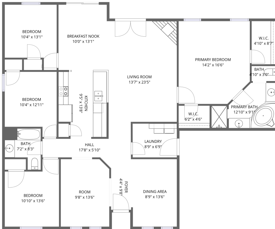
1st floor
