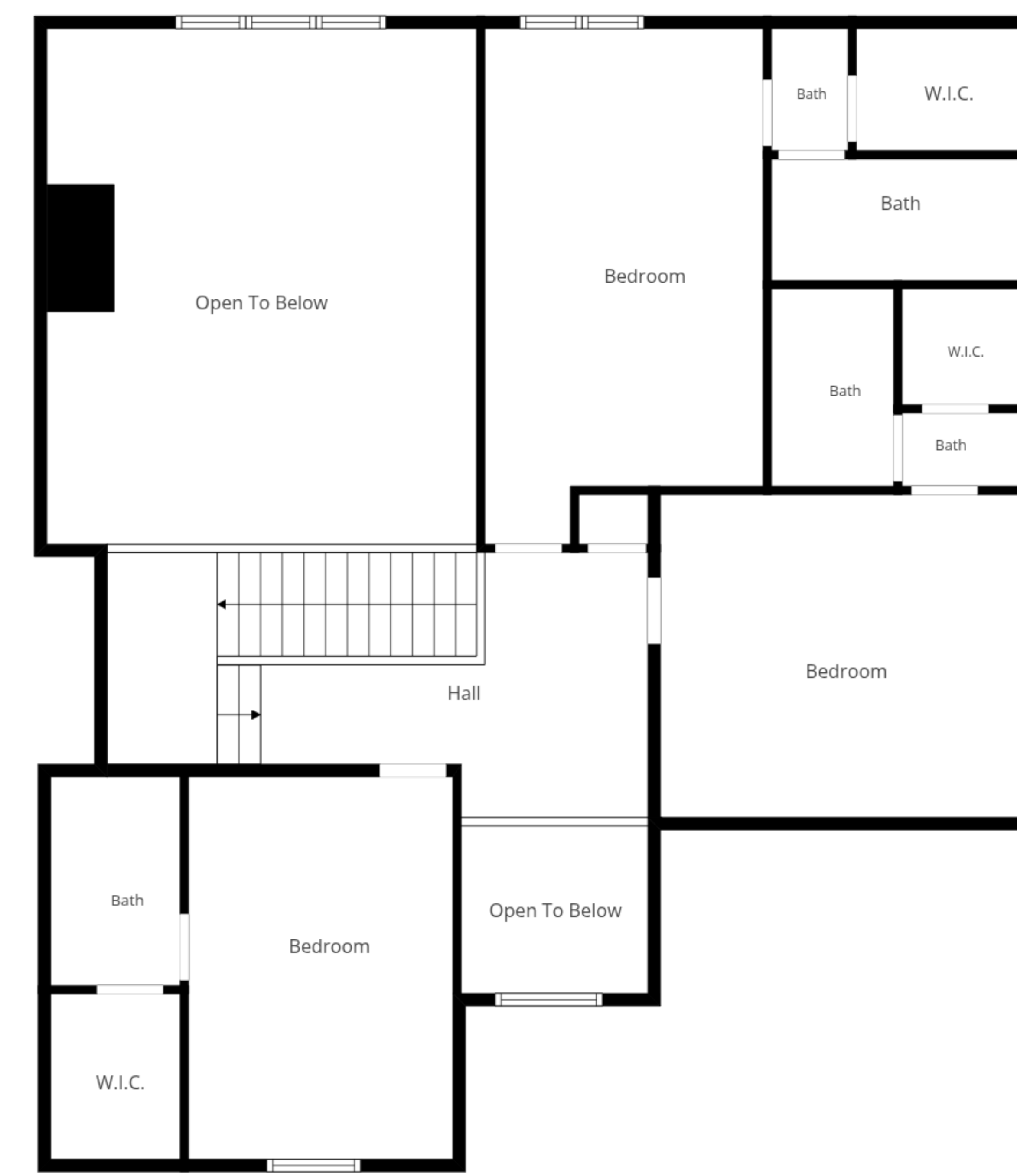
2nd Floor
