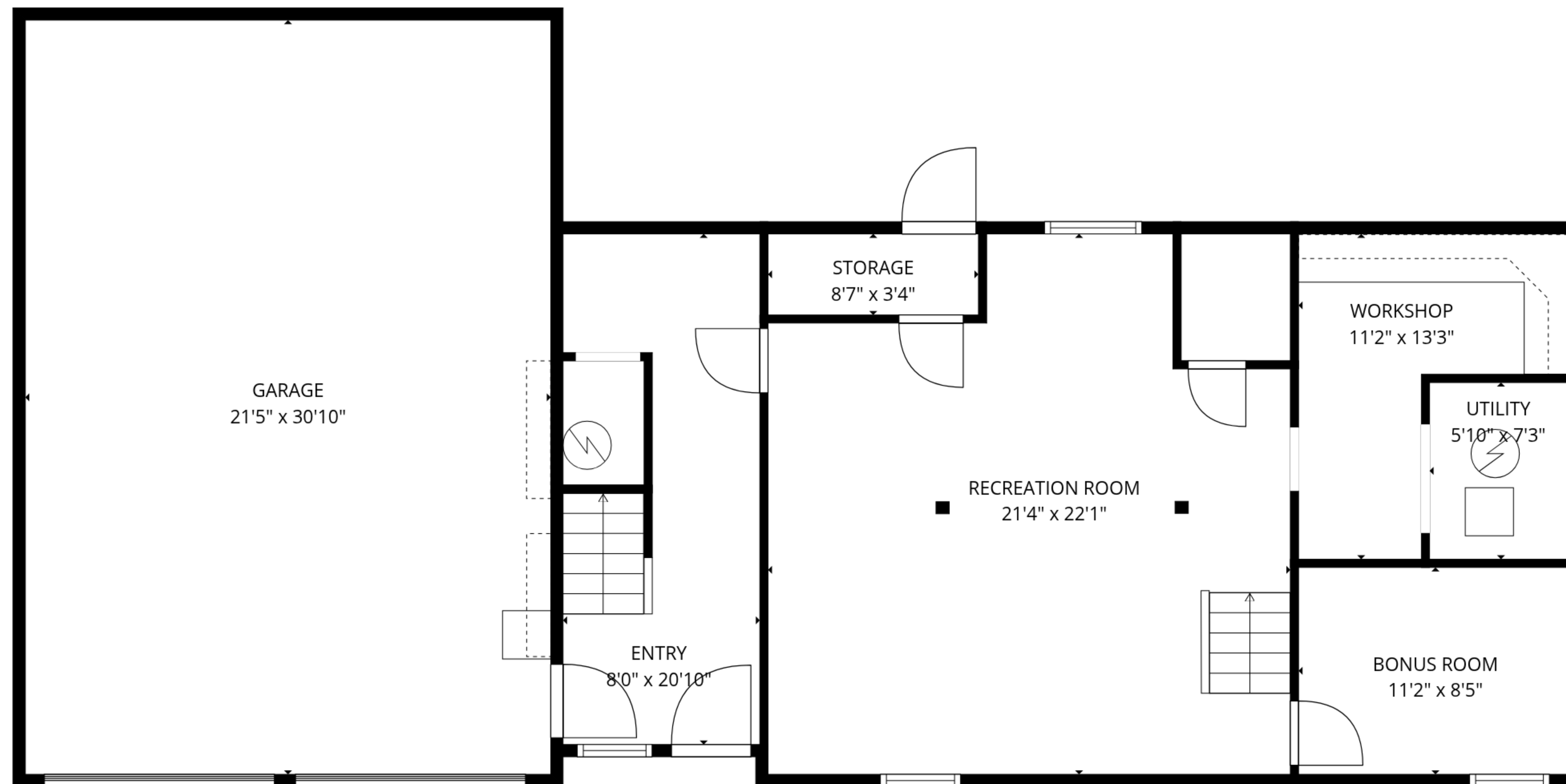
FLOOR 2
