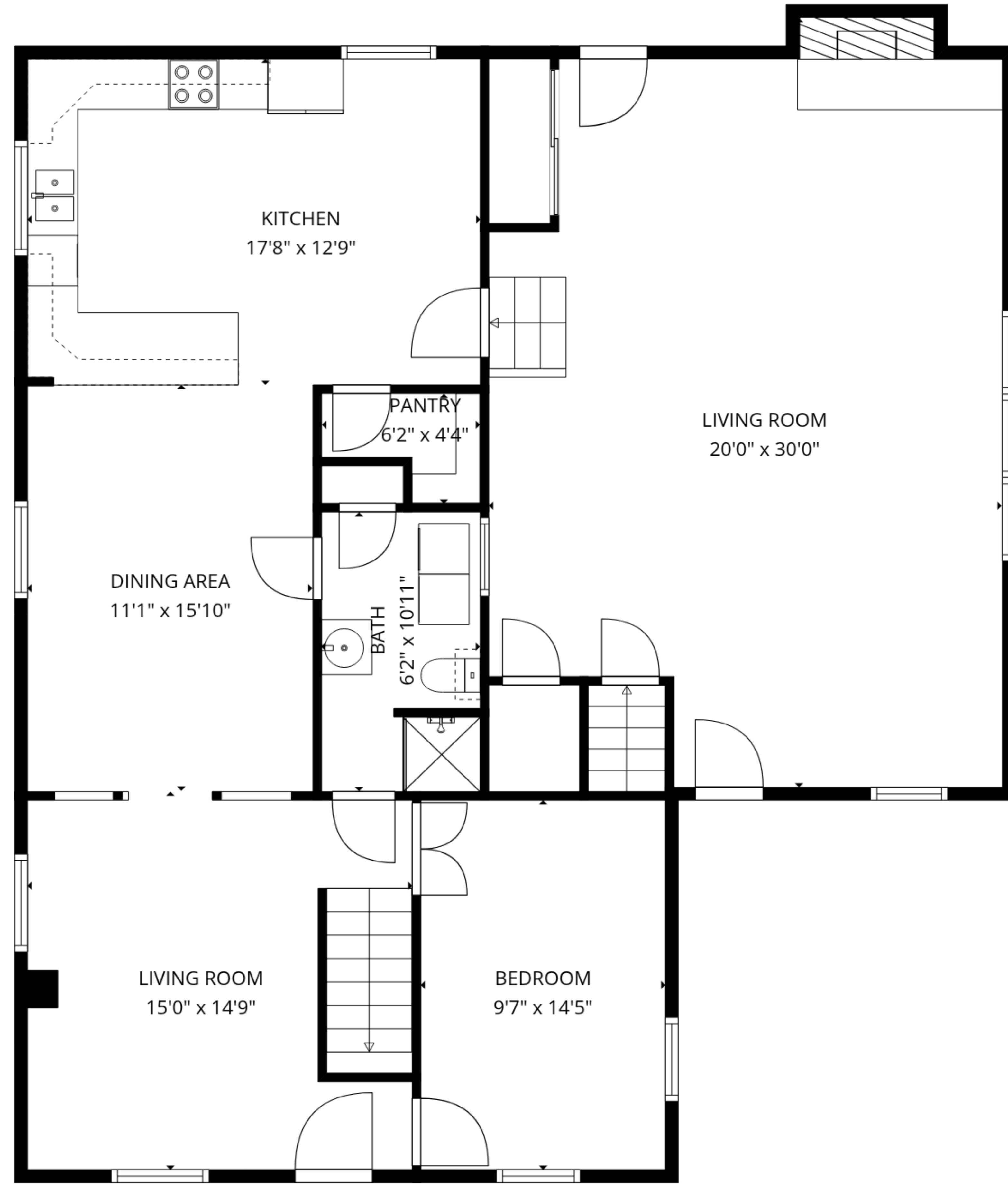
1st floor
