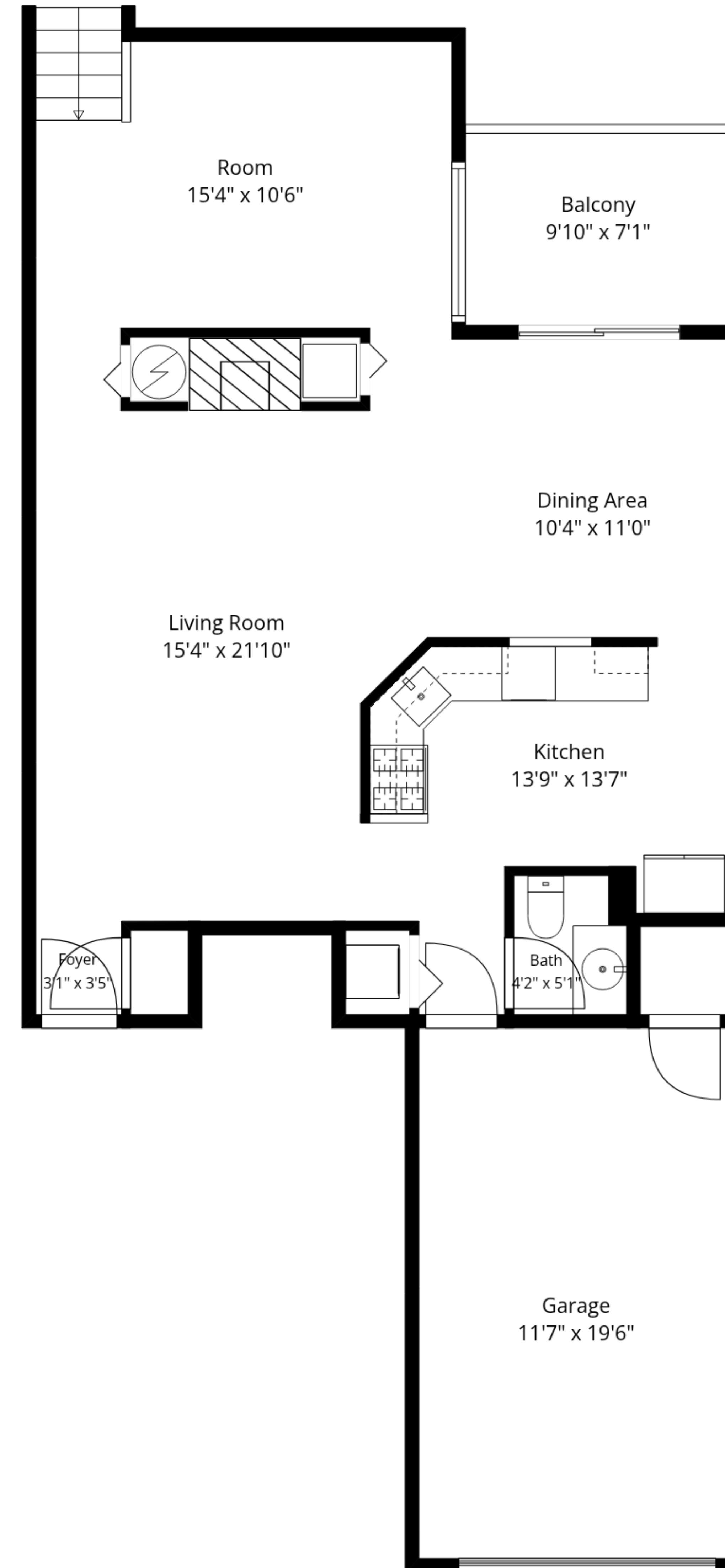
2nd Floor
