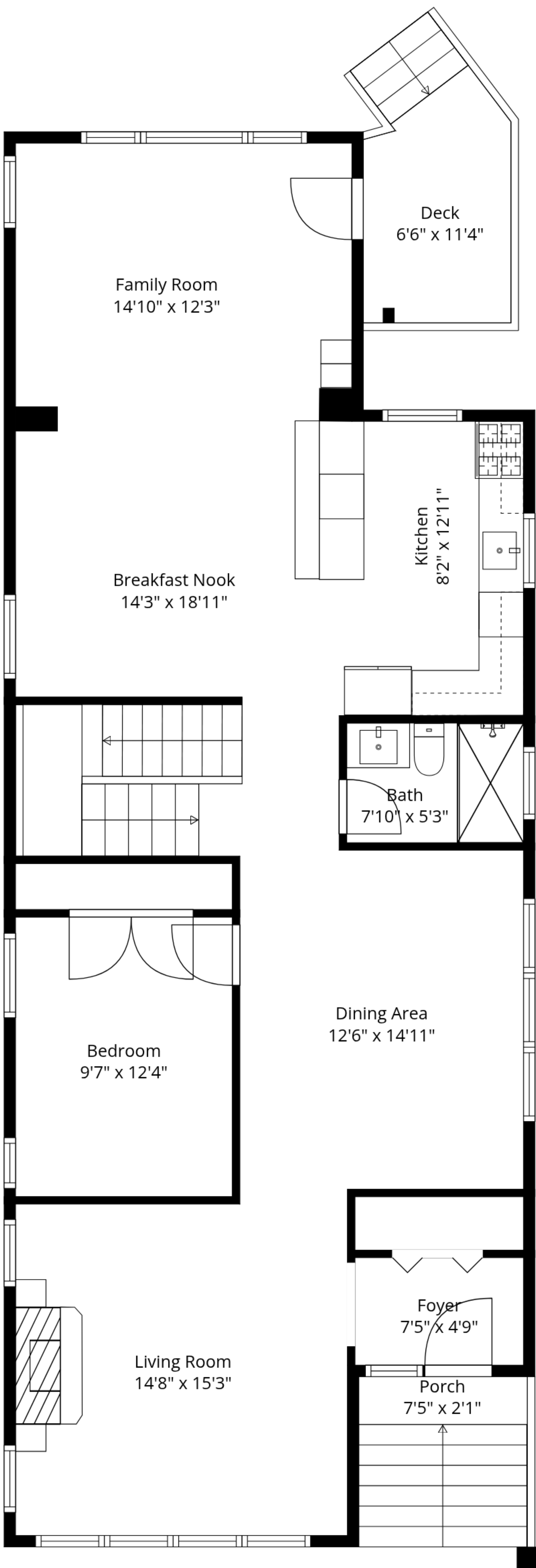
2nd Floor
