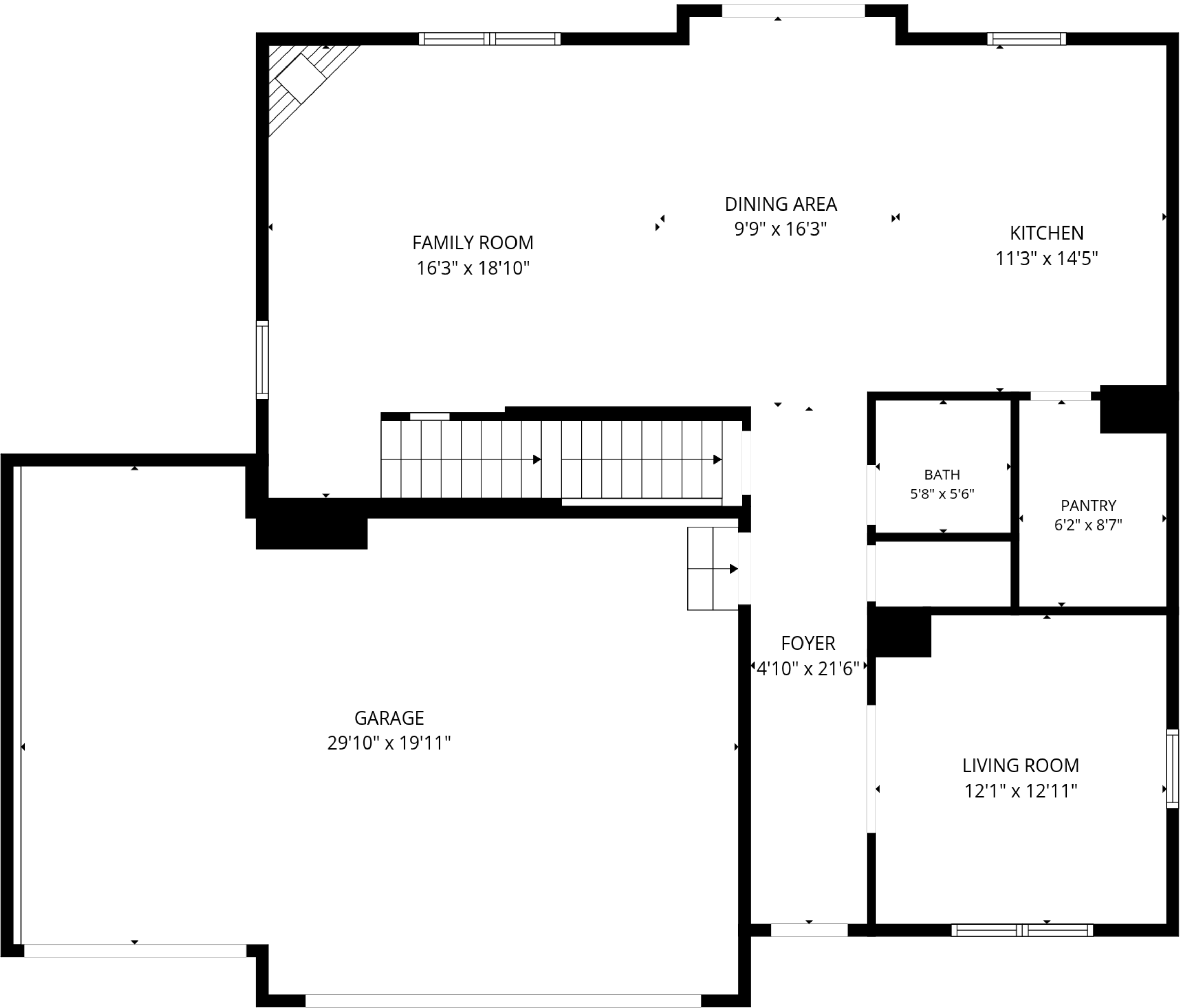
1st floor
