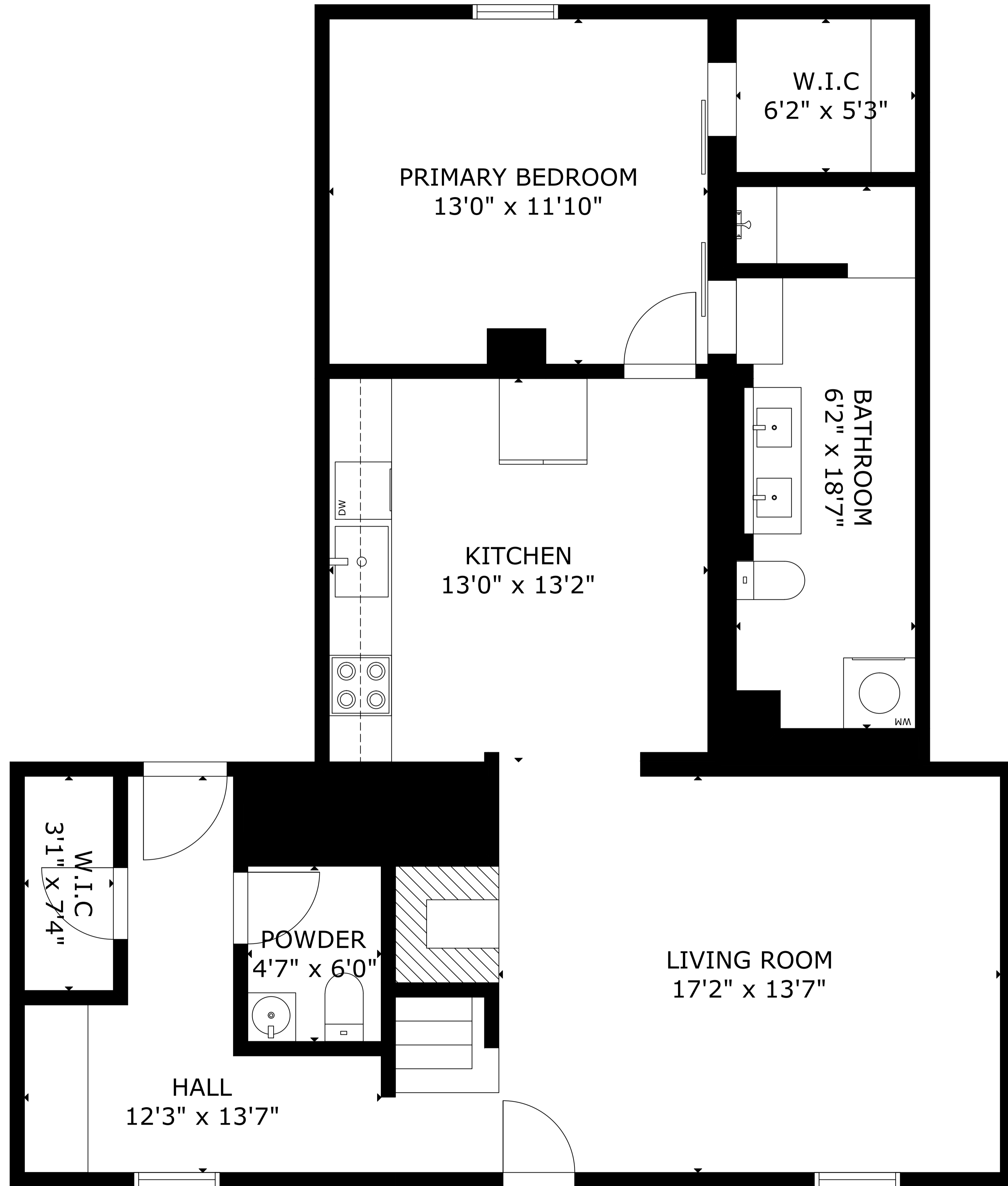
FLOOR 1
