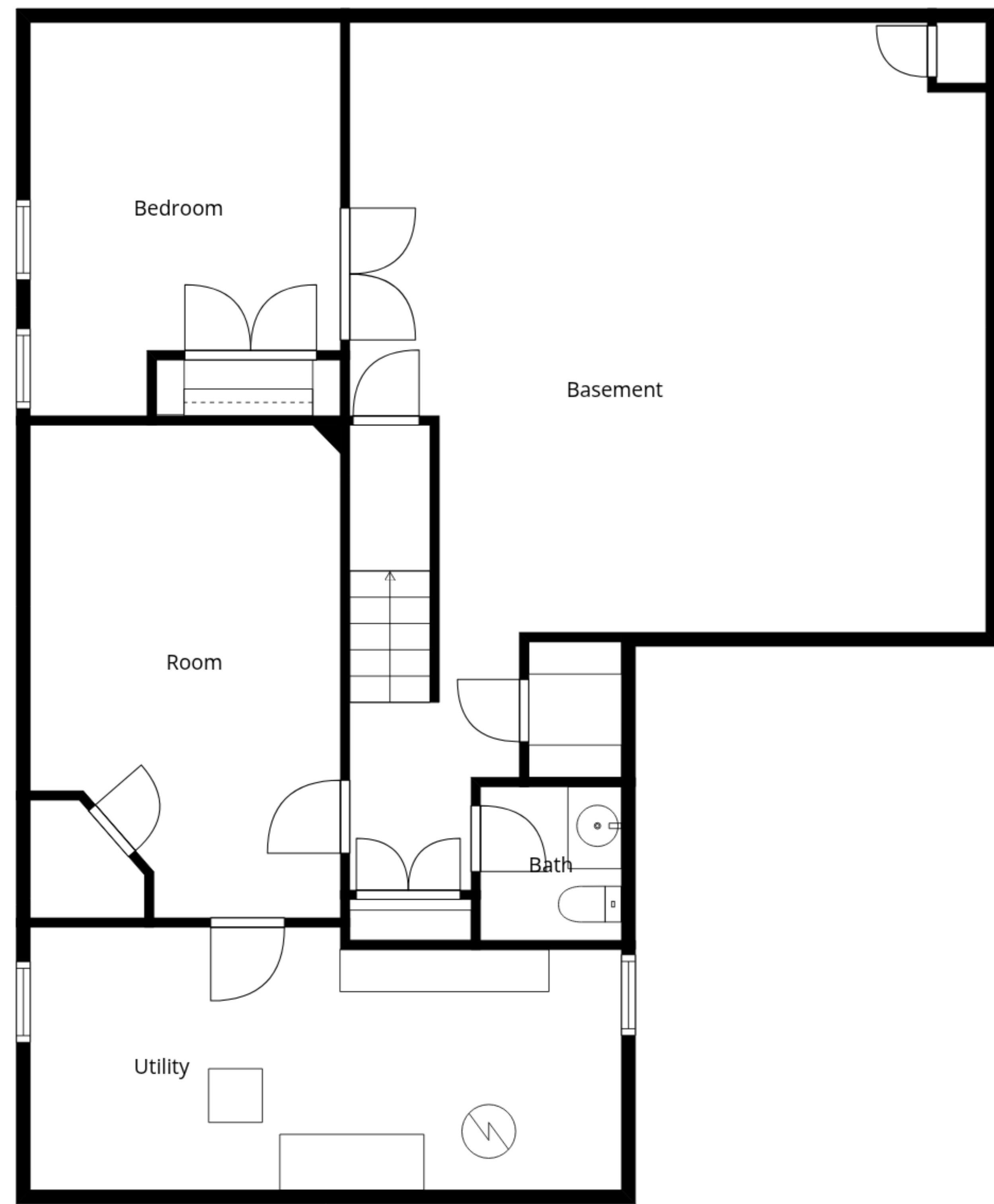
Basement
