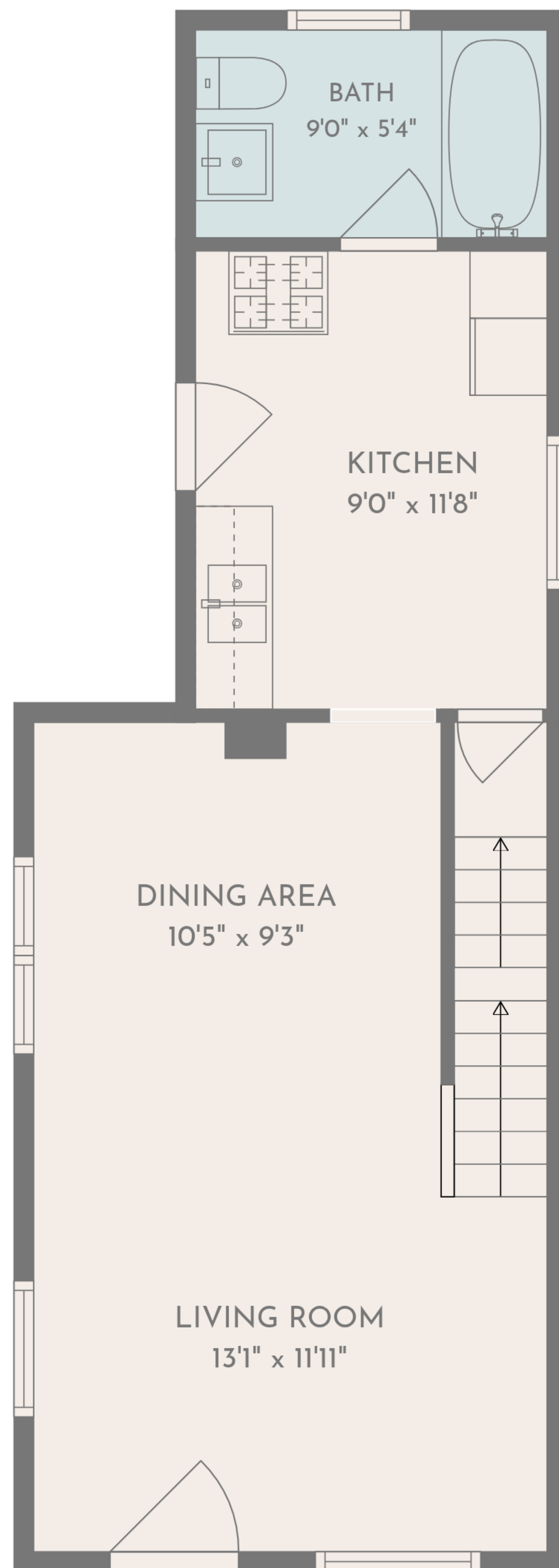
1st floor
