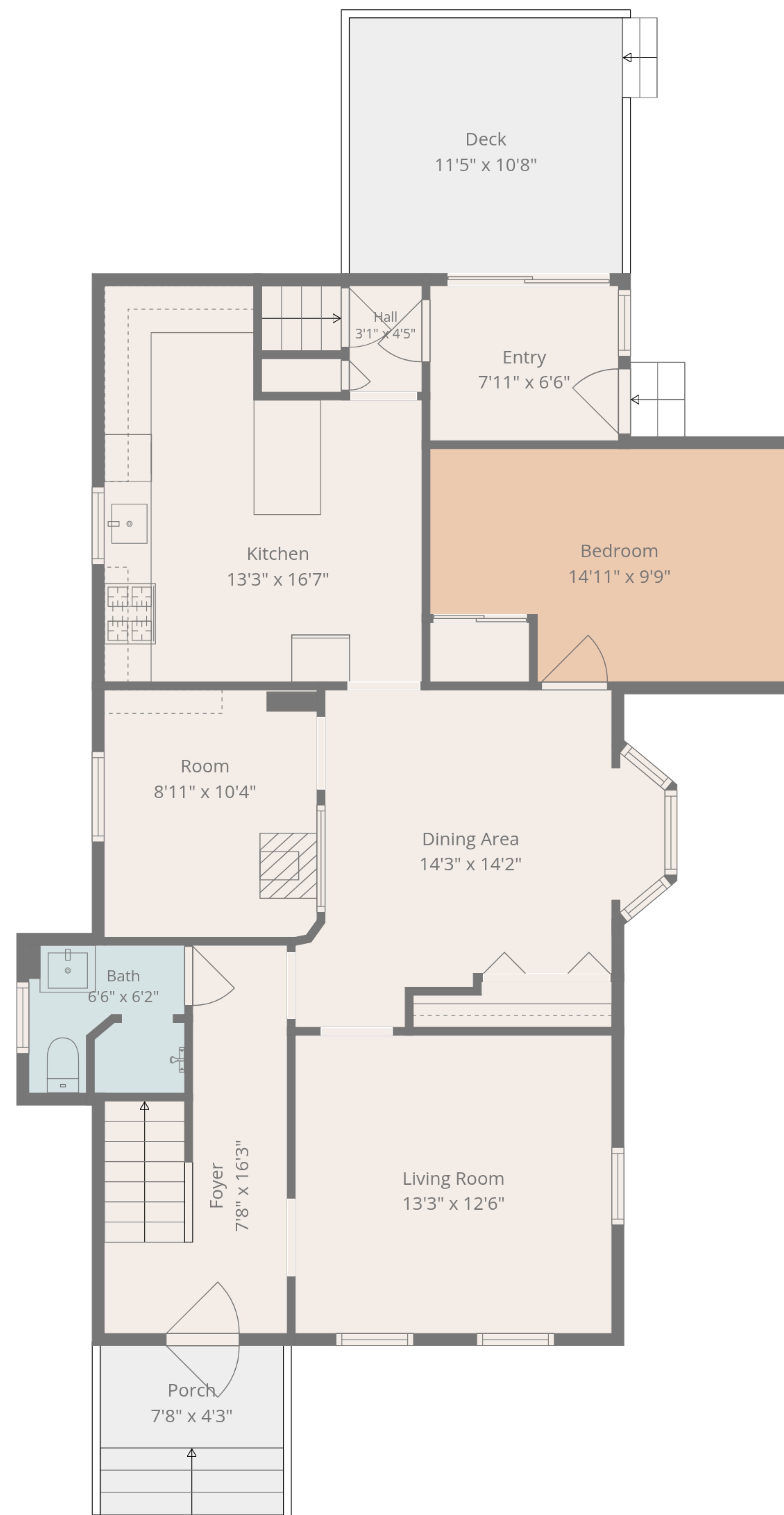
1st Floor
