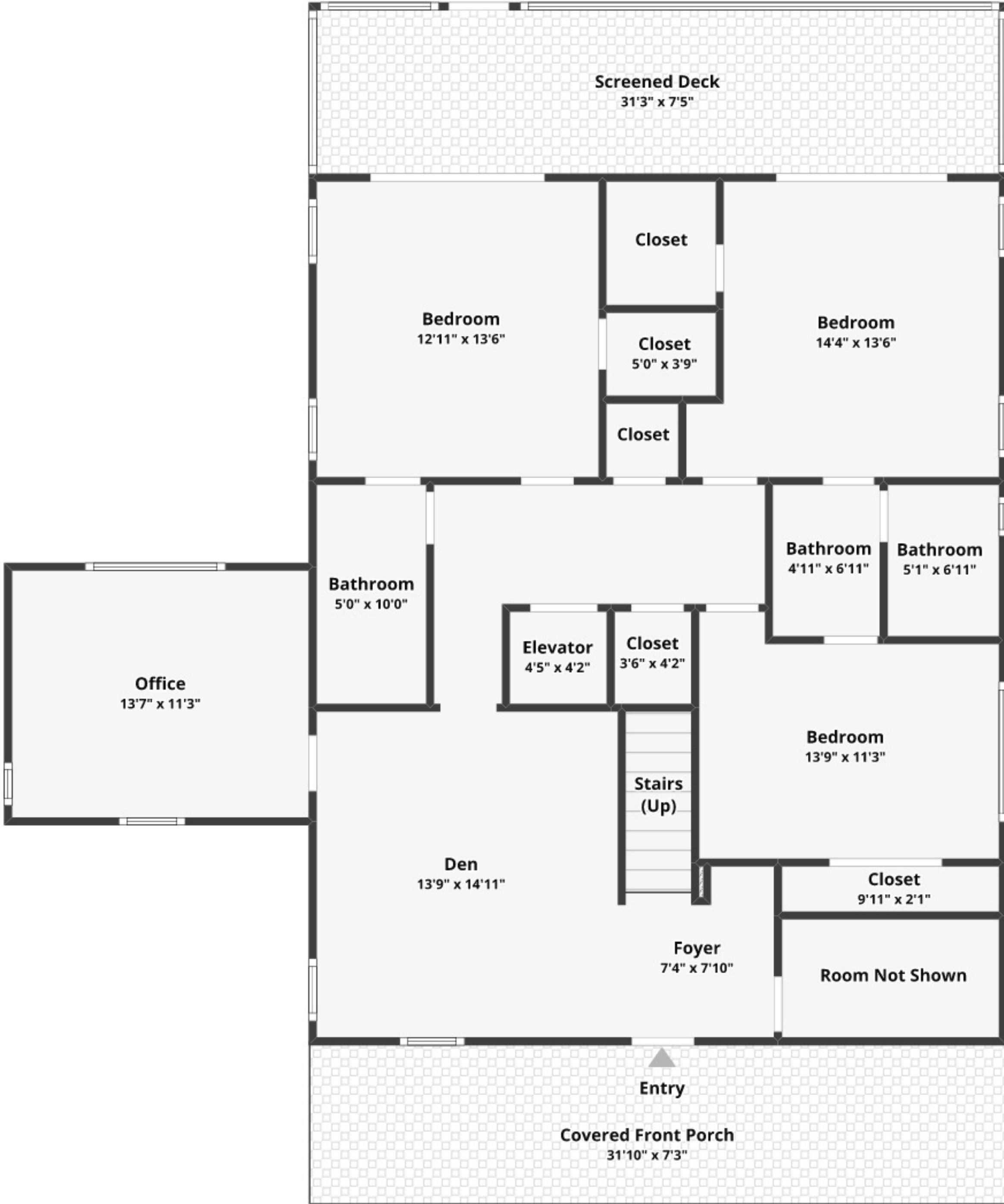
FLOOR 1
