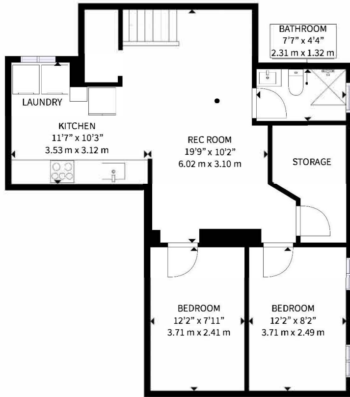
BASEMENT 1
