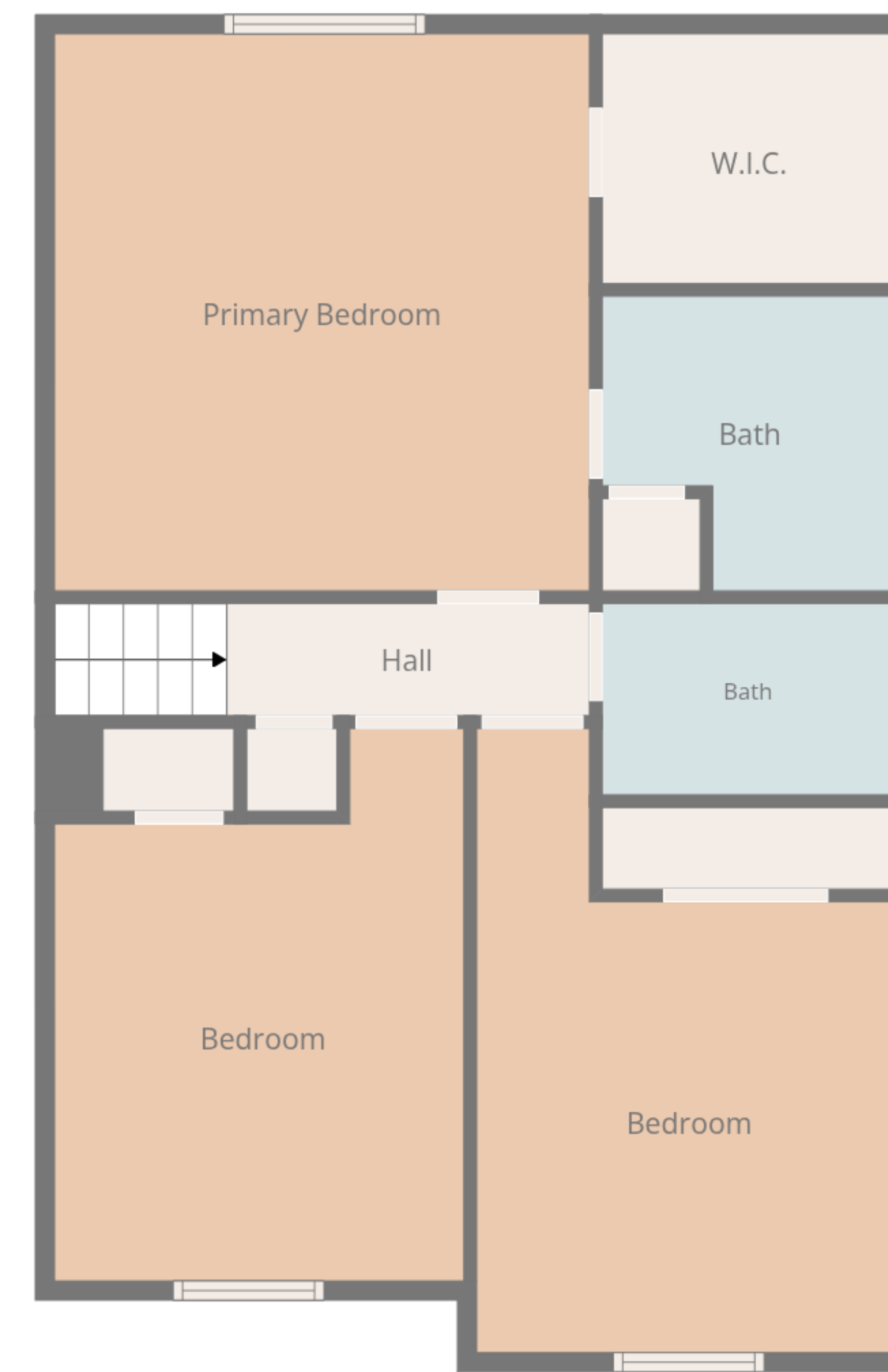
3rd Floor
