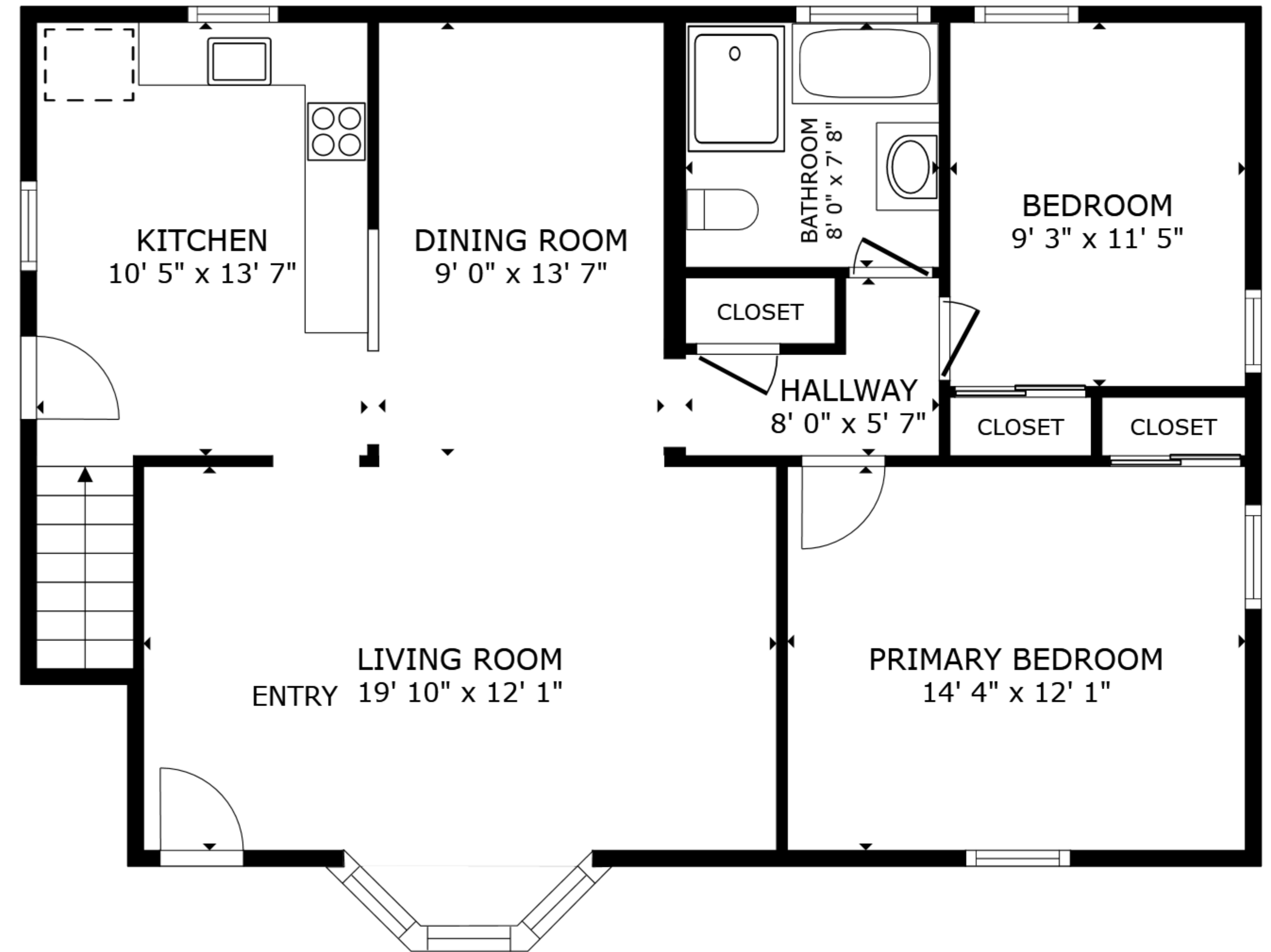
FLOOR 2
