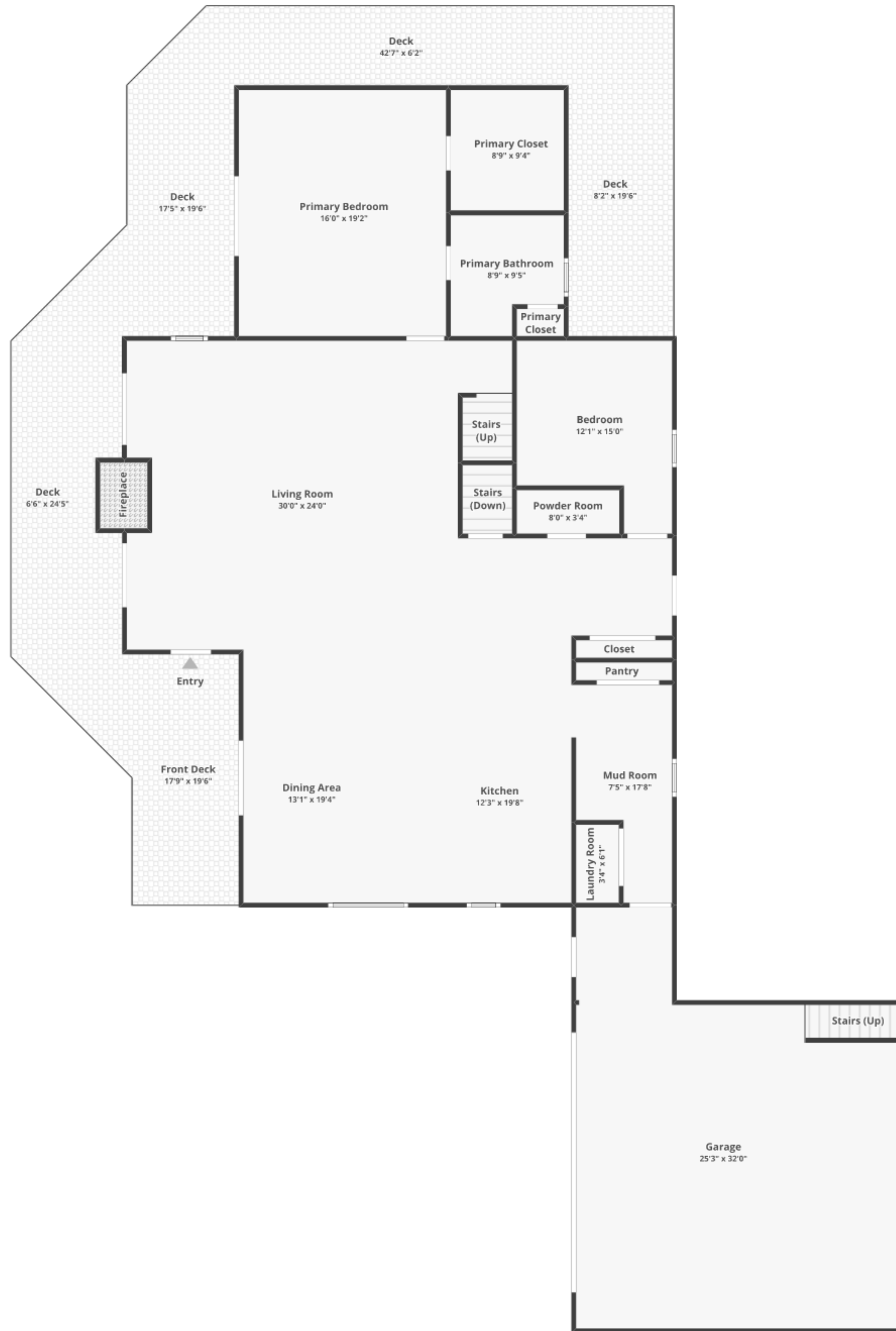
FLOOR 1 Finished area: ~2,072.35 sq. ft. Unfinished area: ~18.73 sq. ft.
