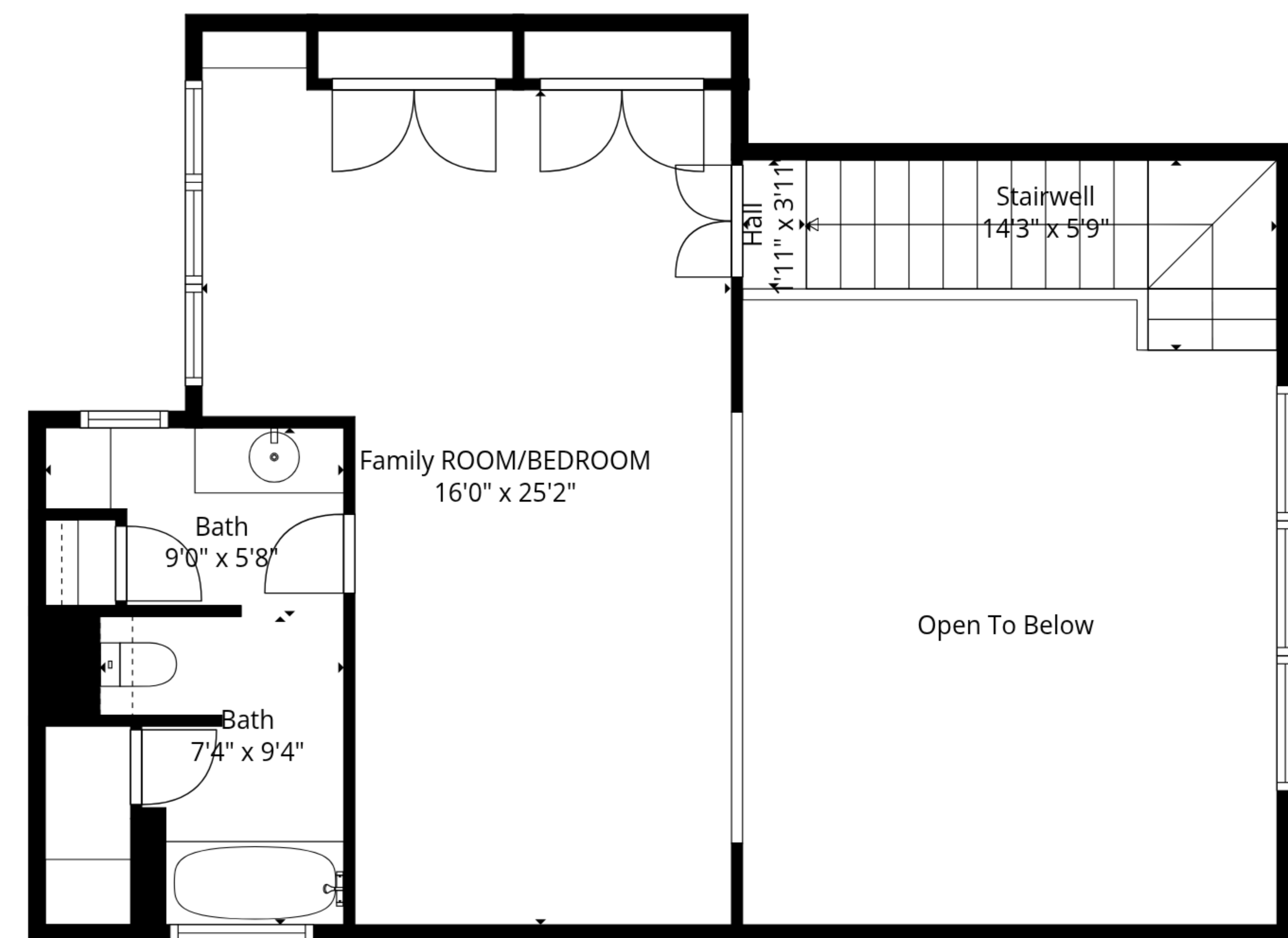
2nd Floor
