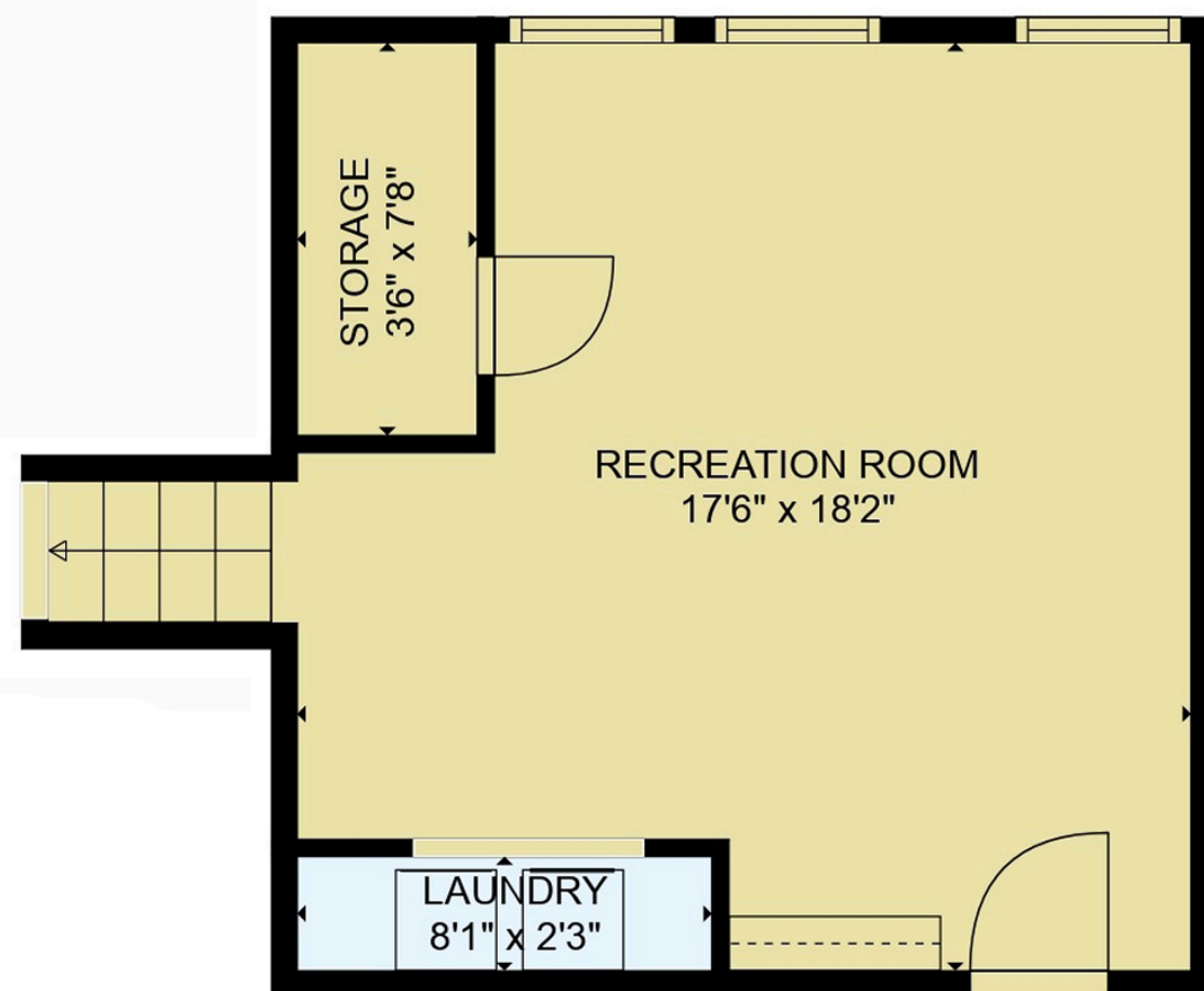
FLOOR 1
