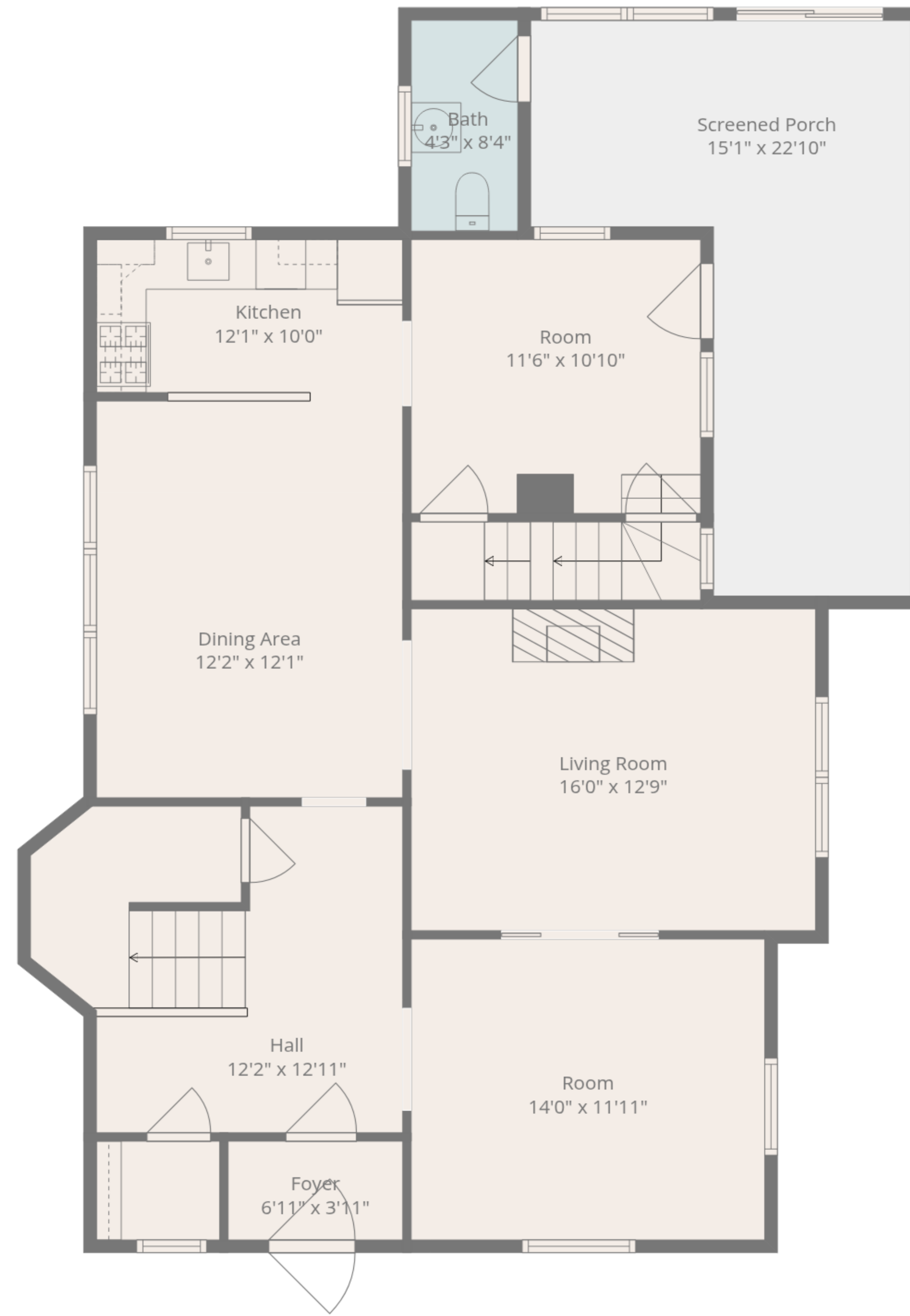
1st Floor
