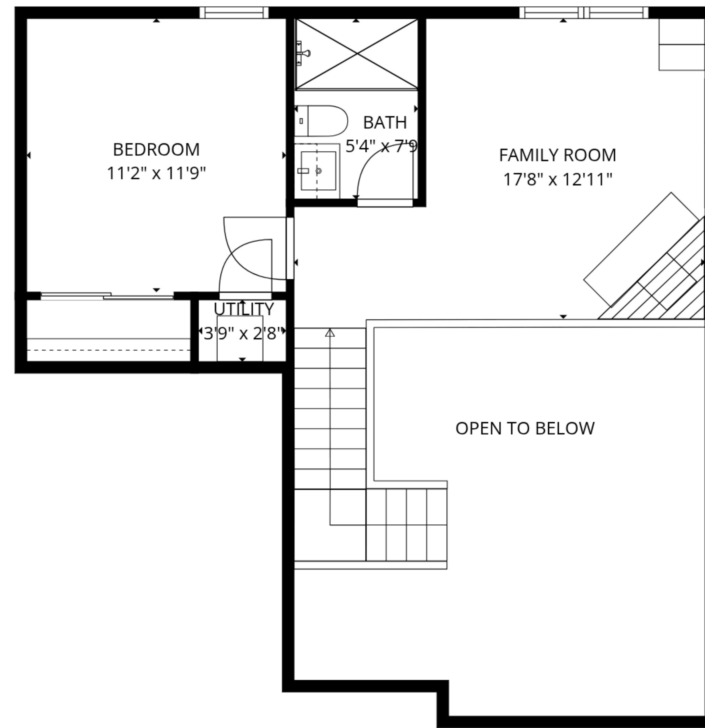
FLOOR 2
