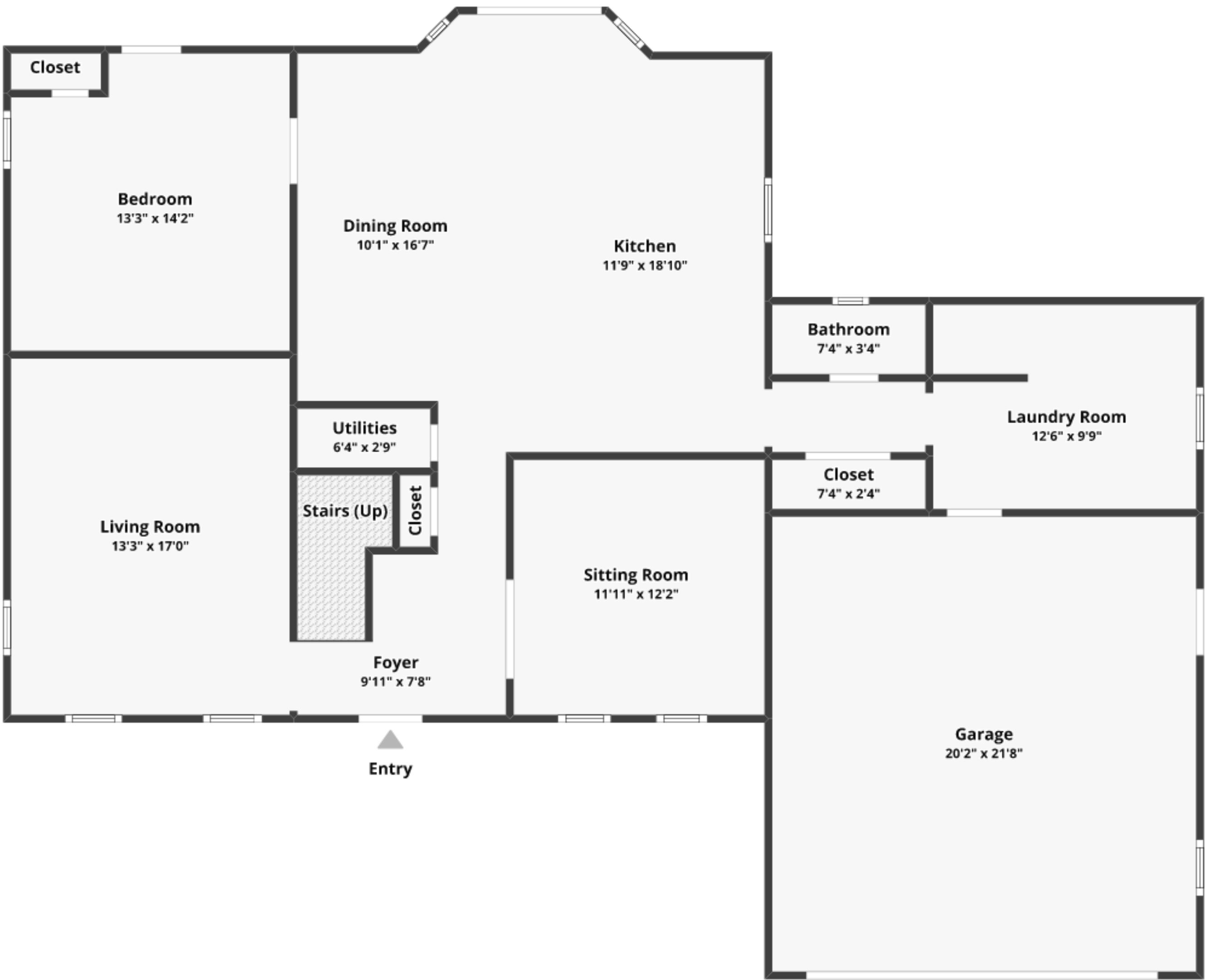
FLOOR 1 Finished area: ~1,266.18 sq. ft.
