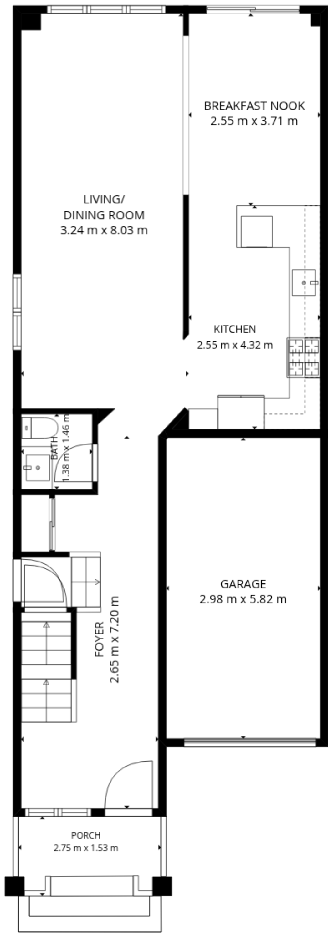
1st floor
