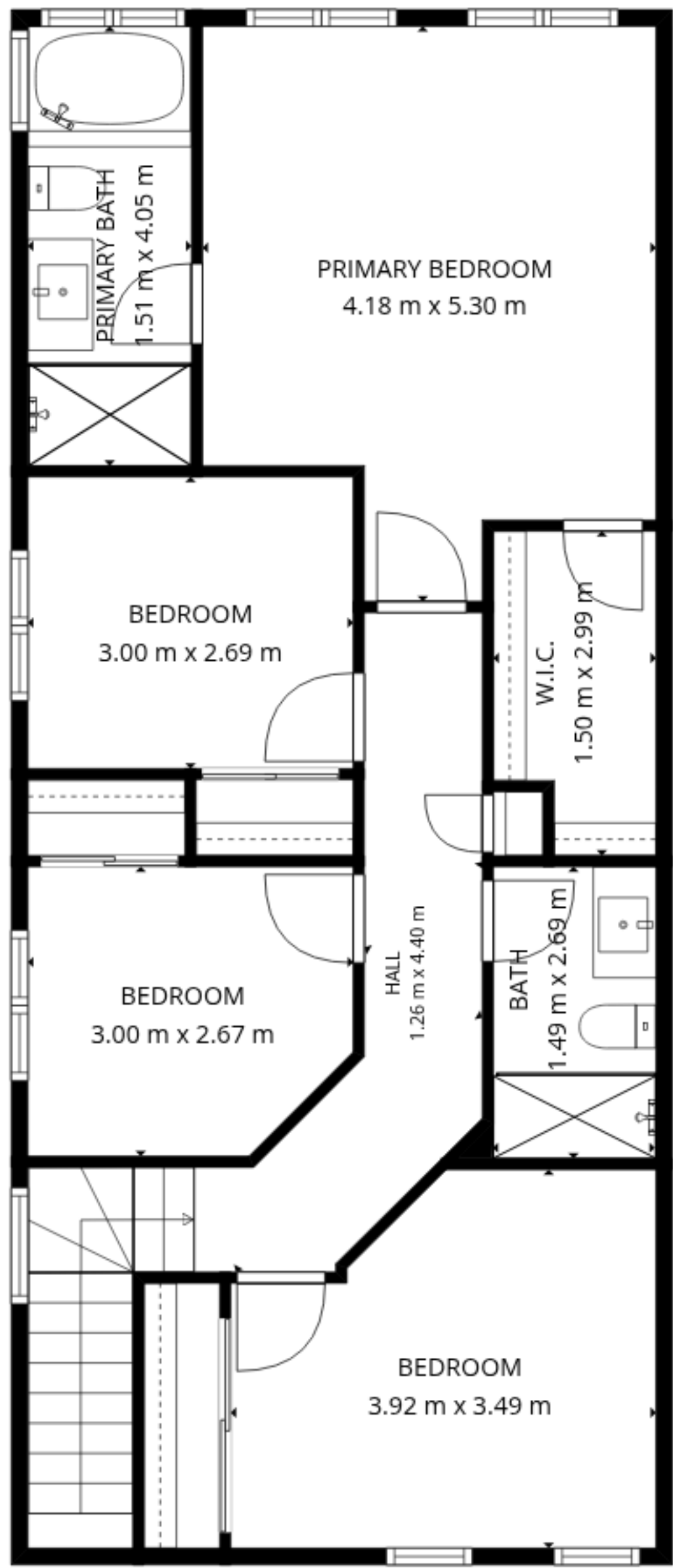
2nd floor
