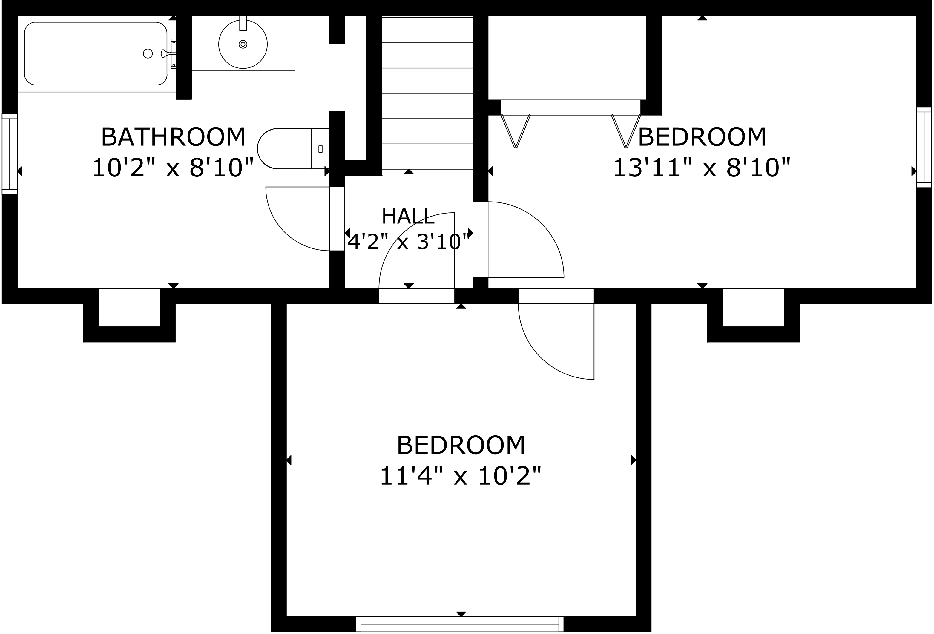
UPPER LEVEL 1
