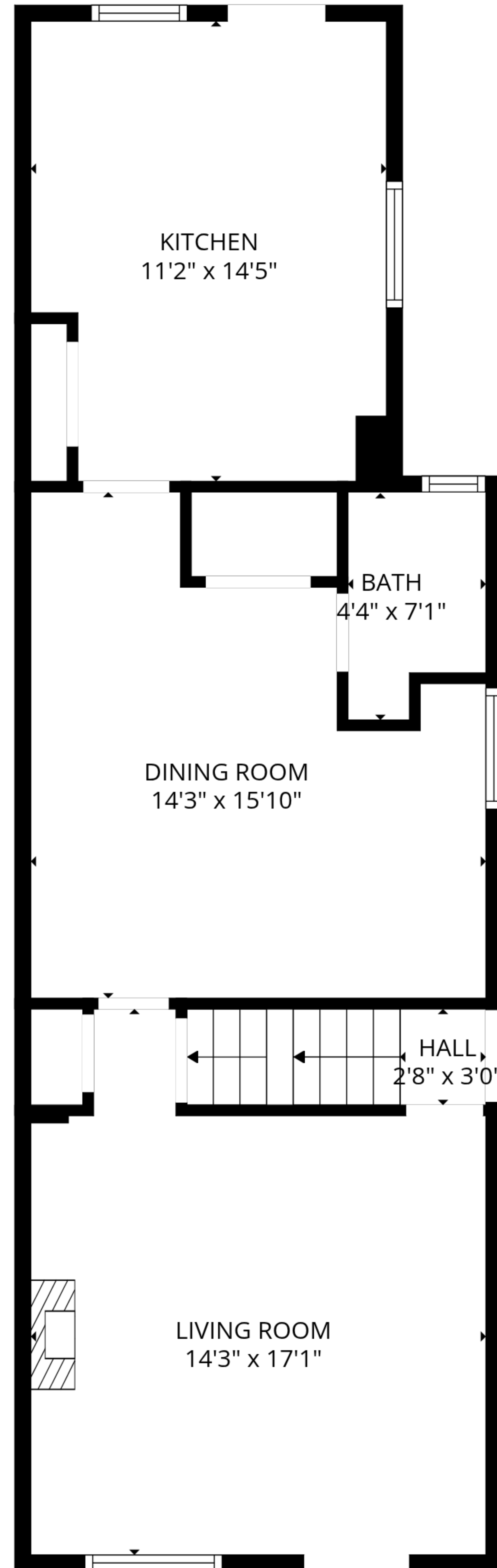
1st floor
