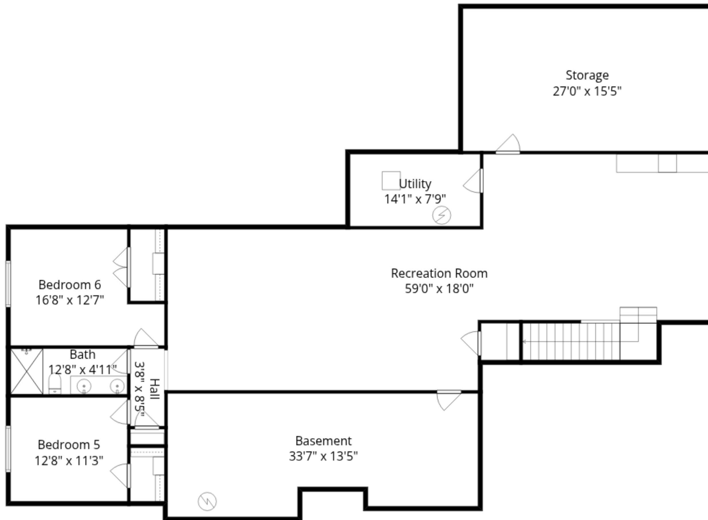
Lower Floor
