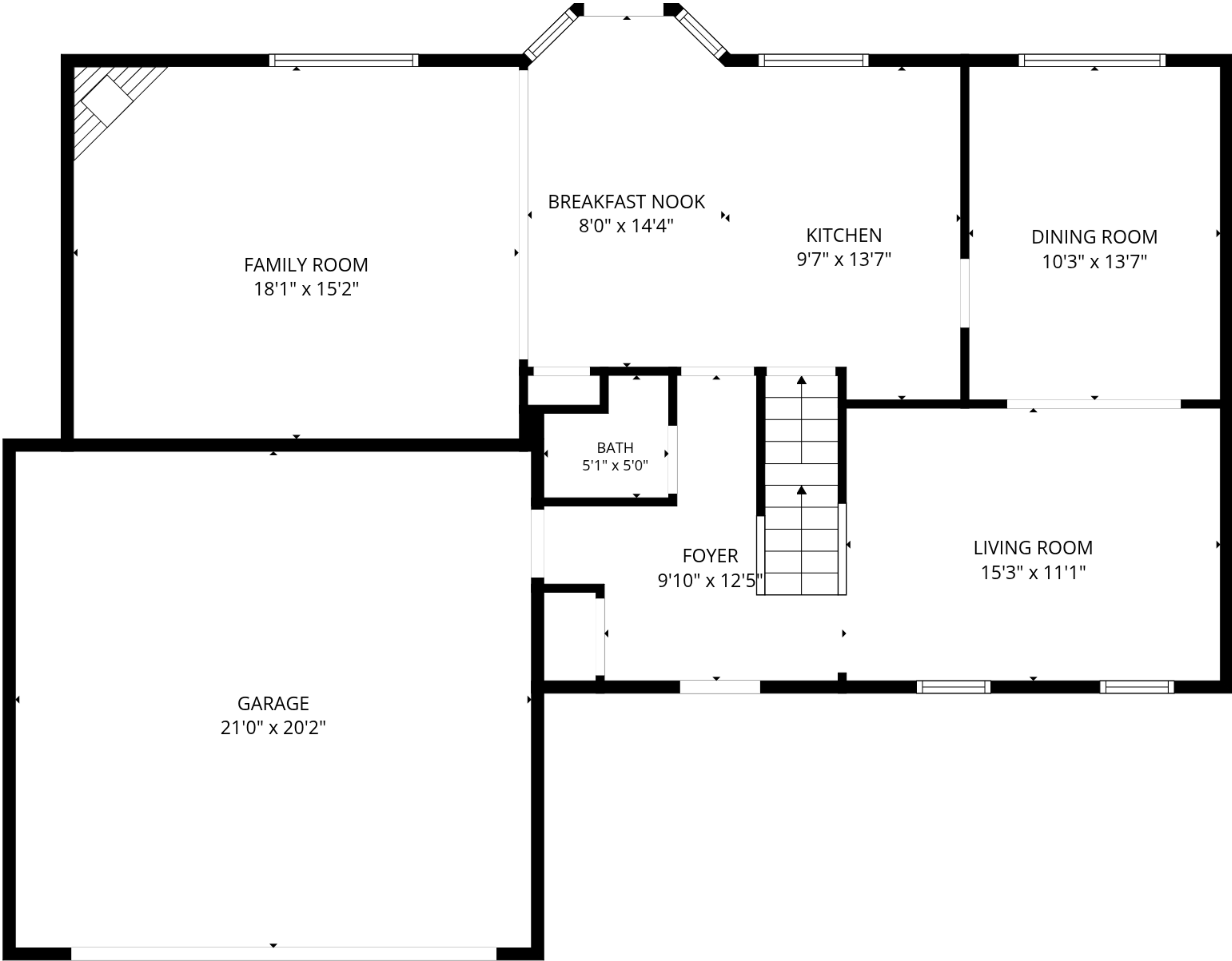
1st floor
