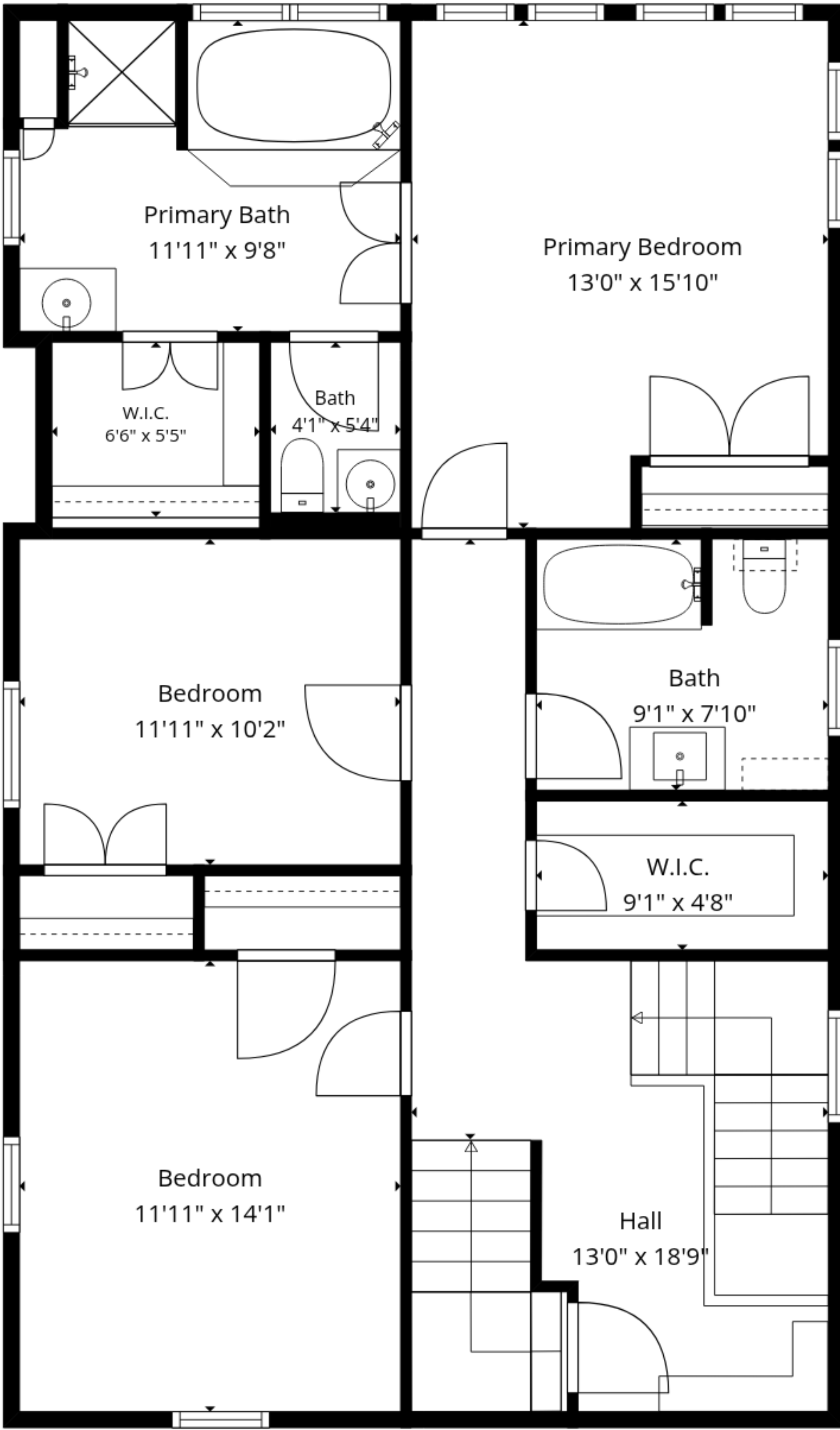
2nd Floor
