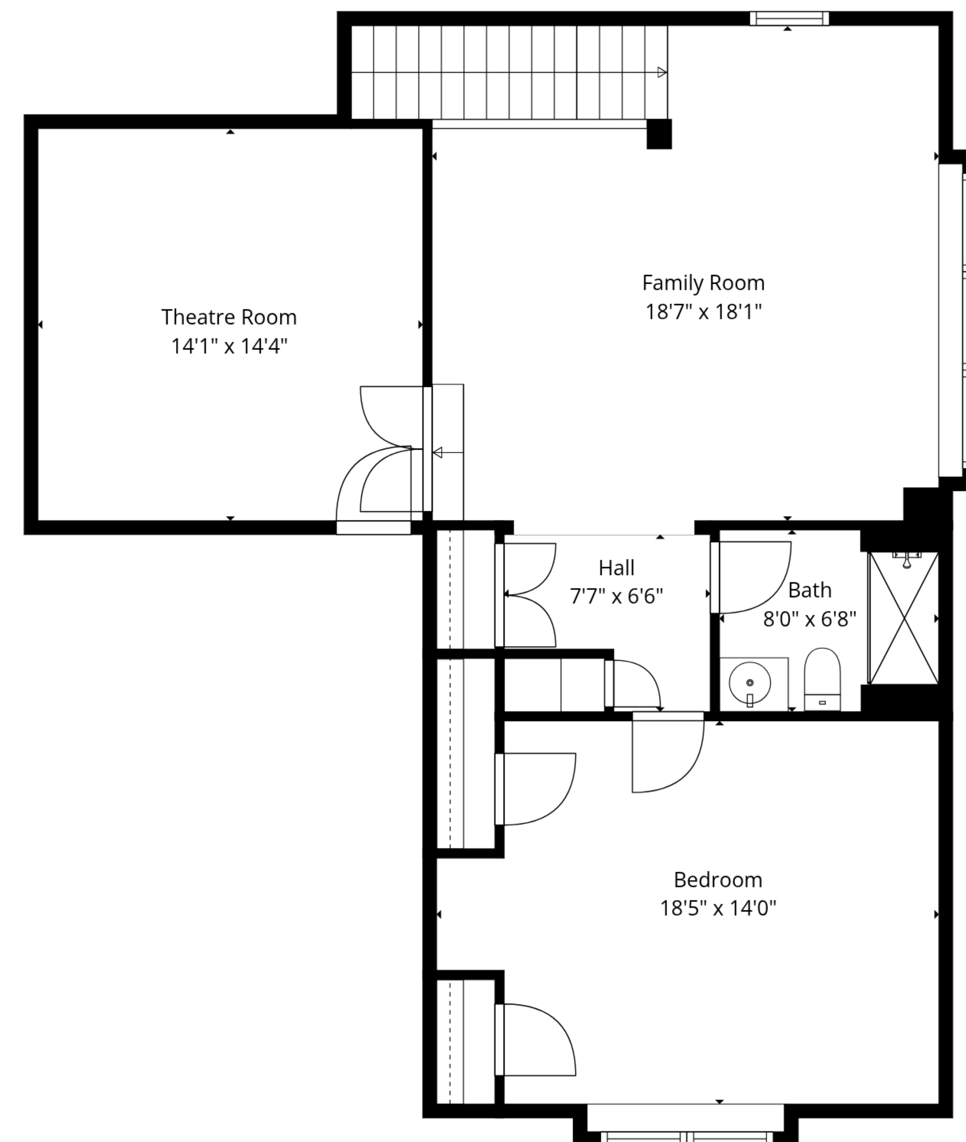
2nd Floor
