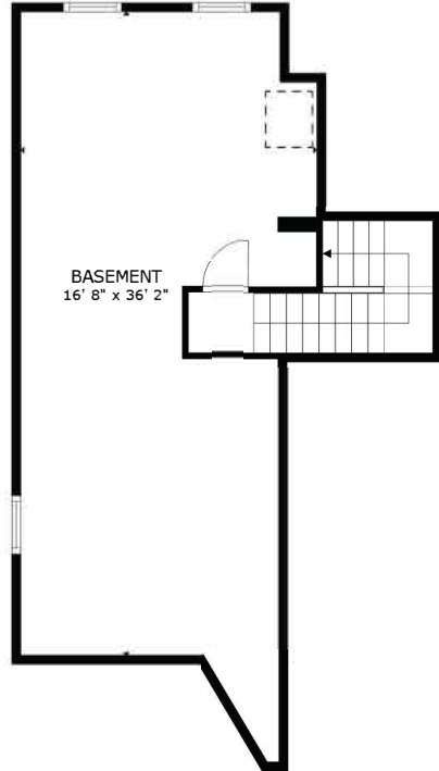
BASEMENT
