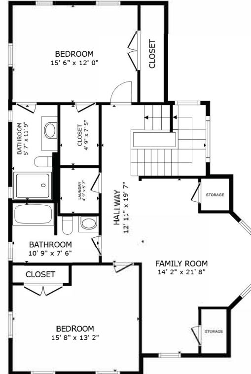
FLOOR 2
