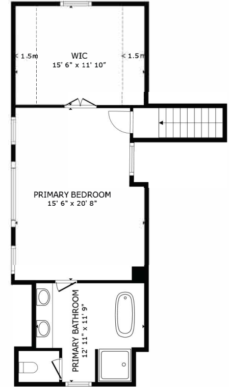
FLOOR 3
