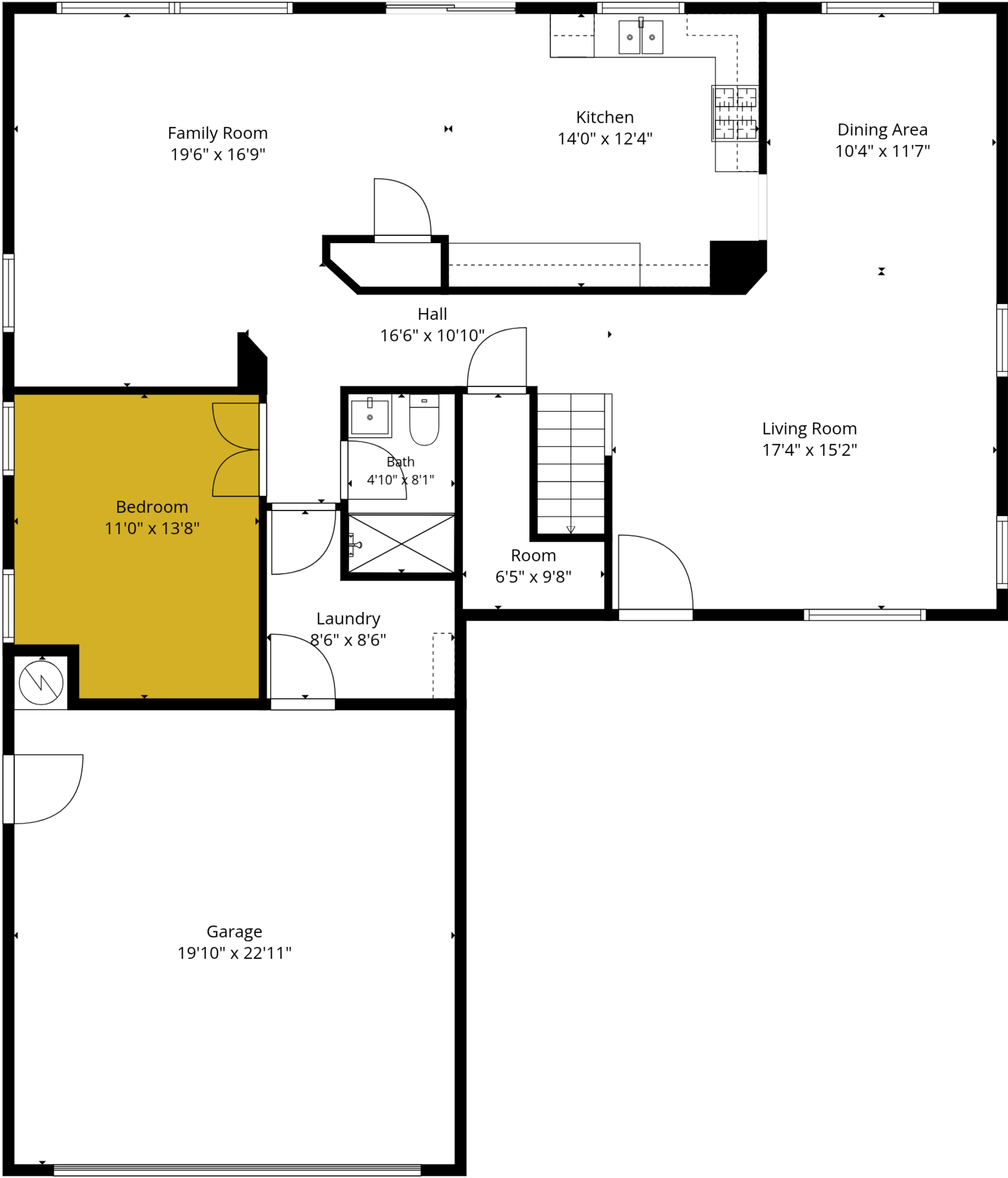
1st Floor
