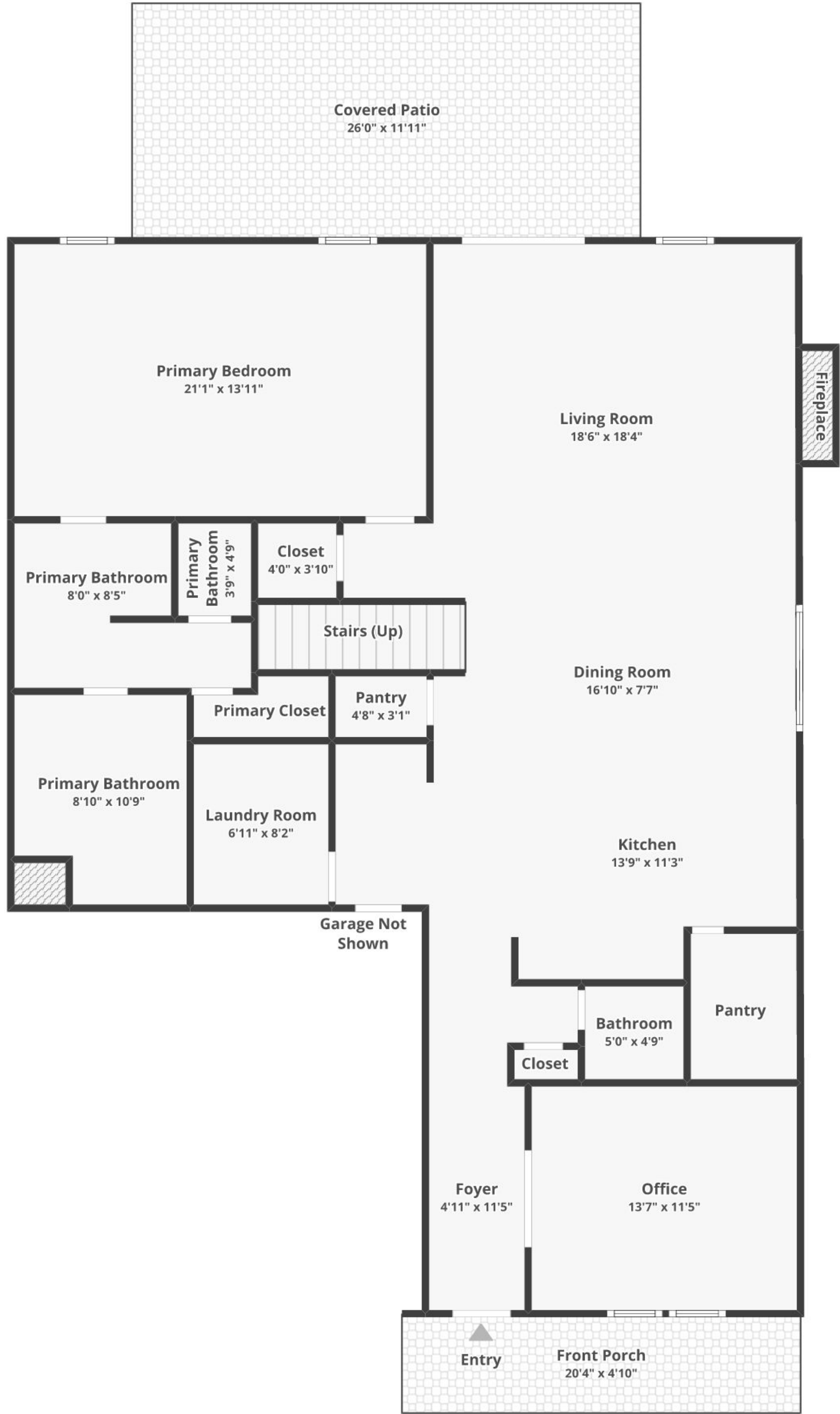
FLOOR 1
