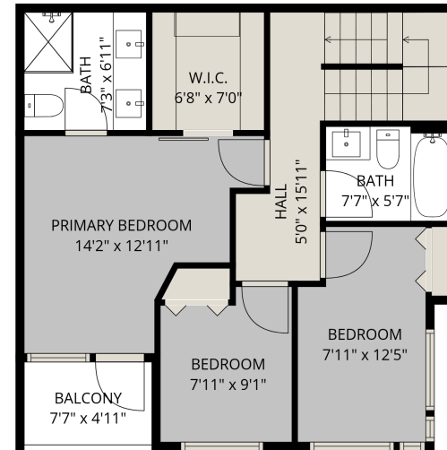
FLOOR 3
