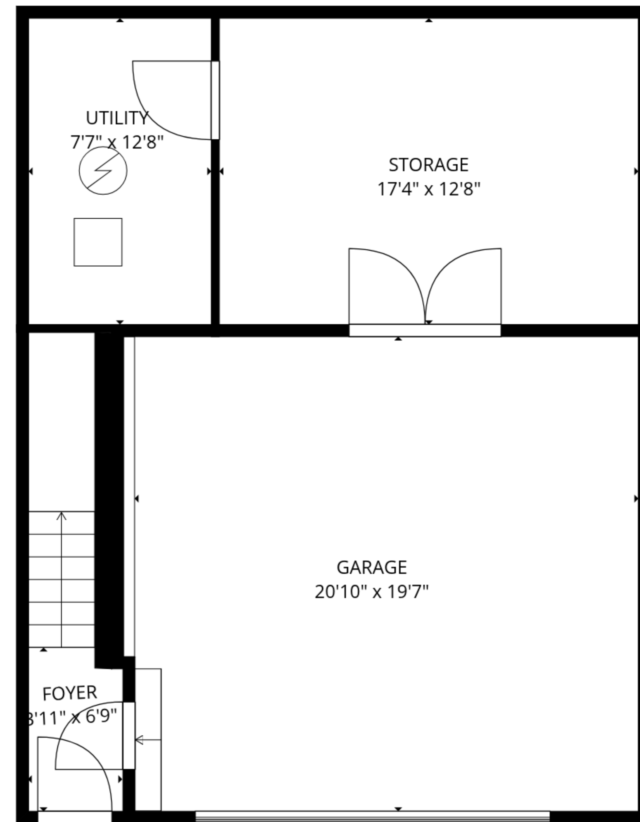
Basement
