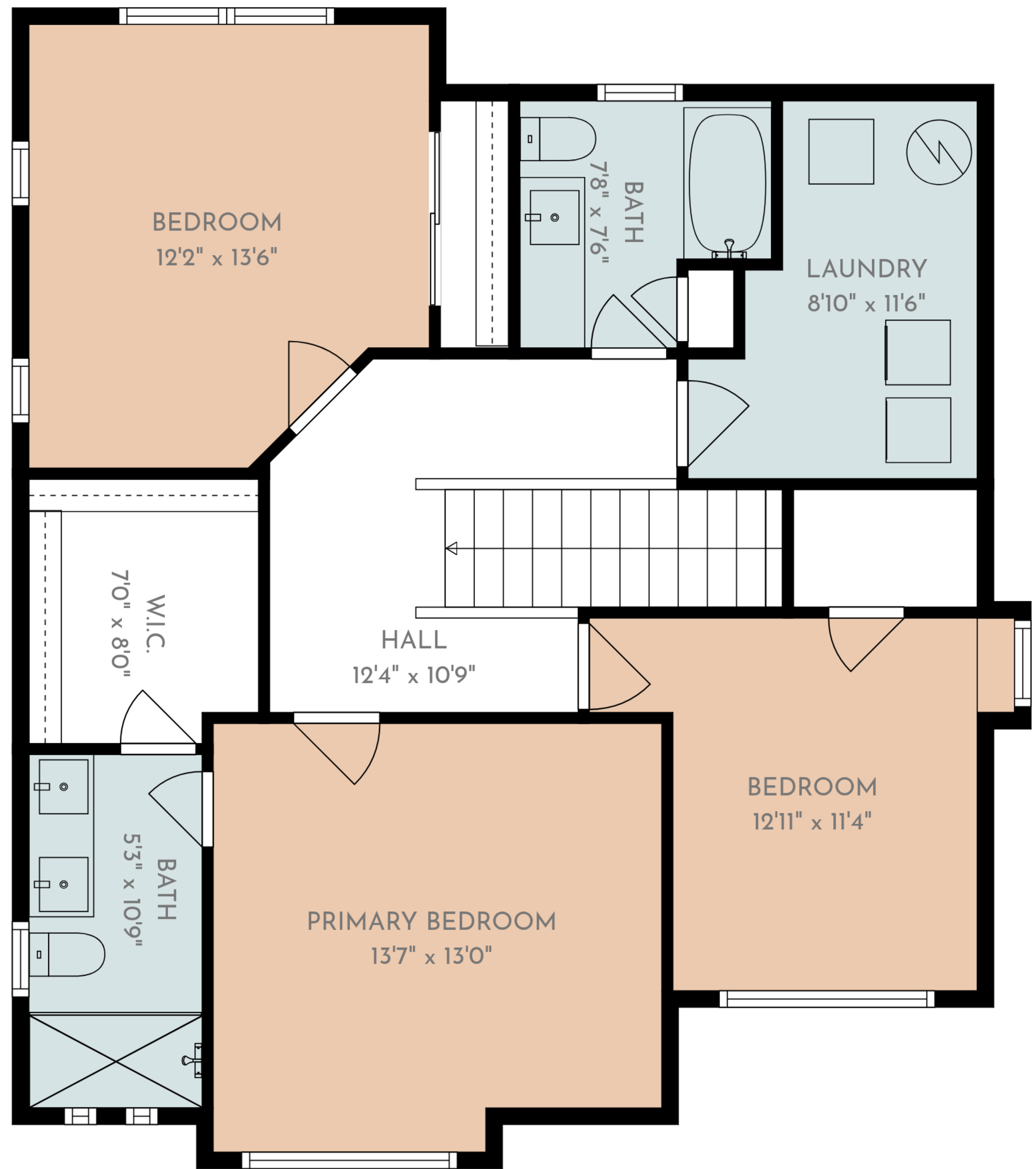
2nd floor
