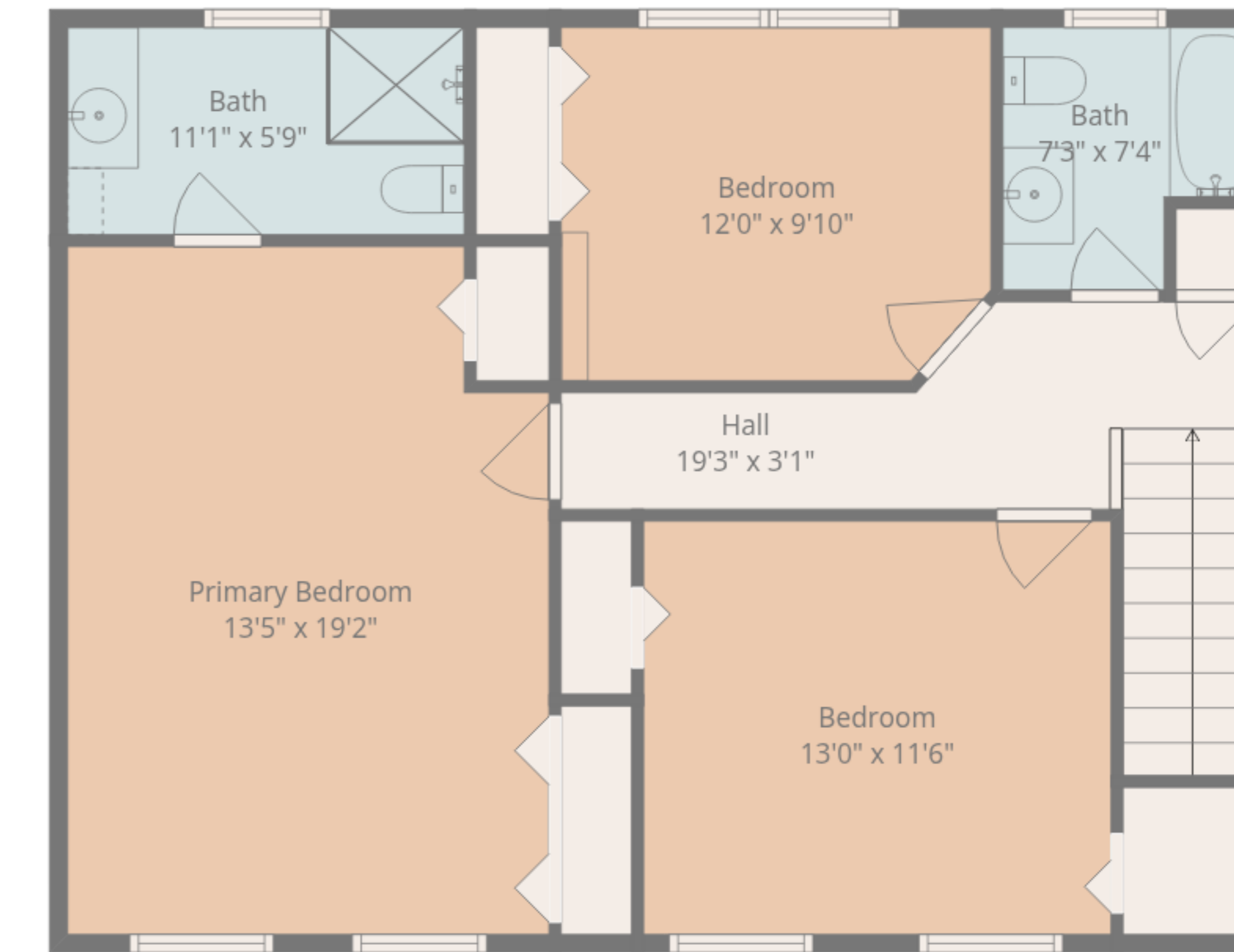
2nd Floor
