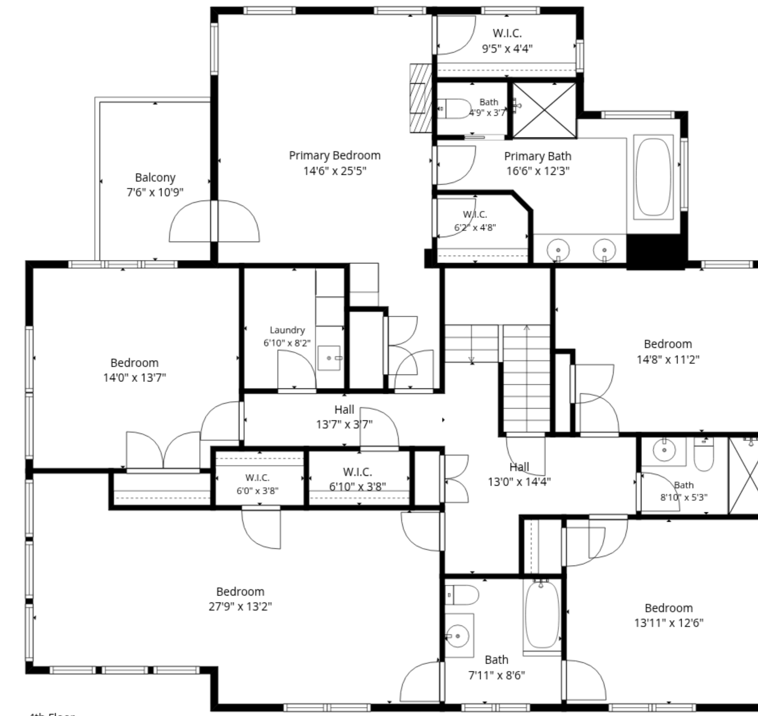
4th Floor
