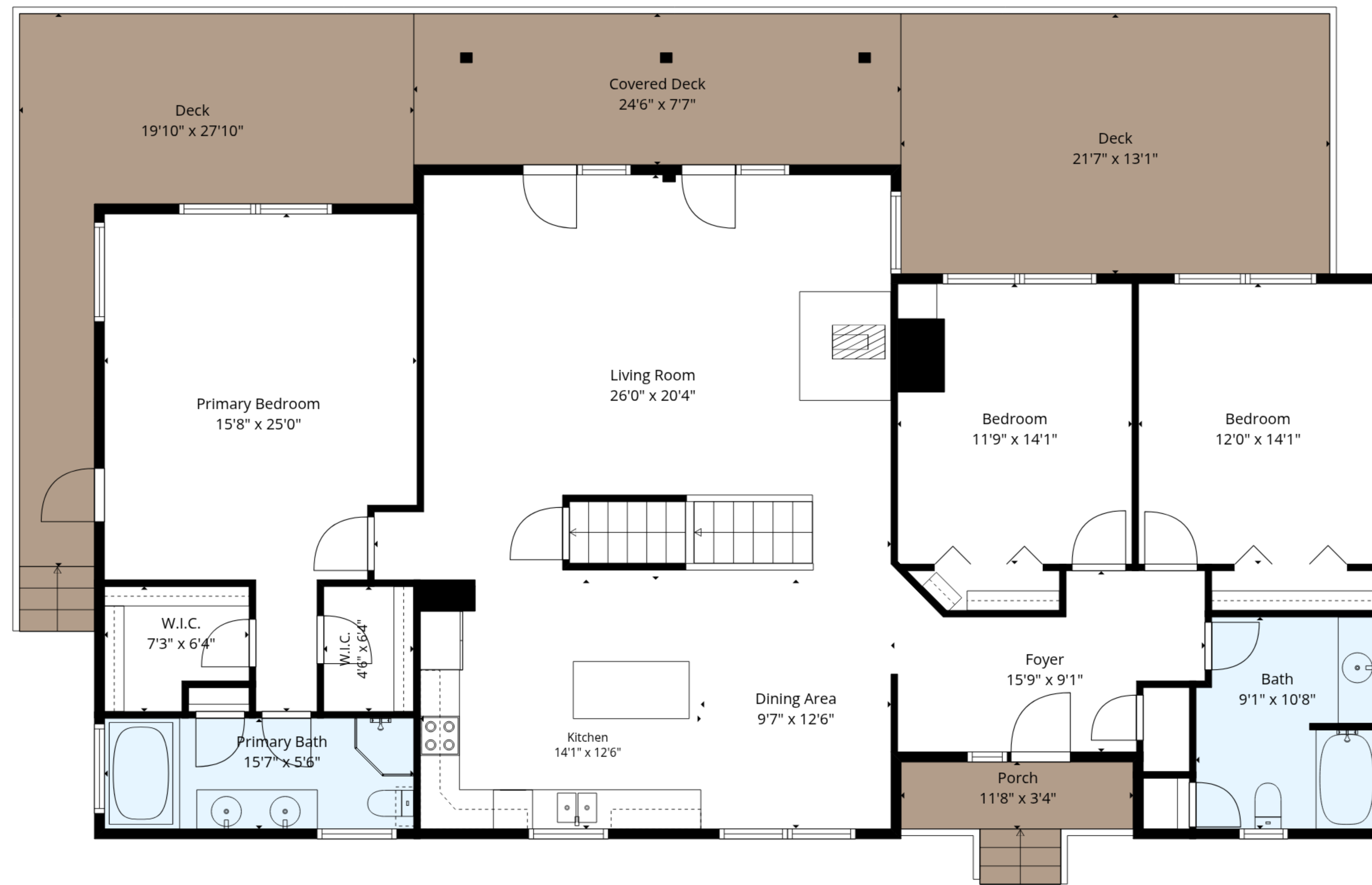
1st Floor
