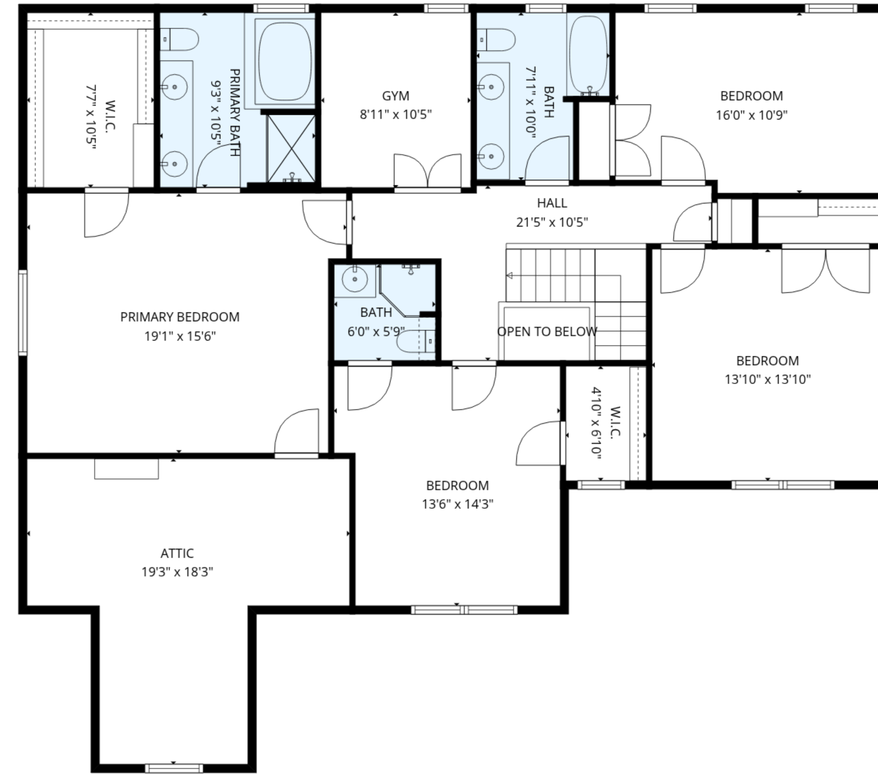
2nd floor
