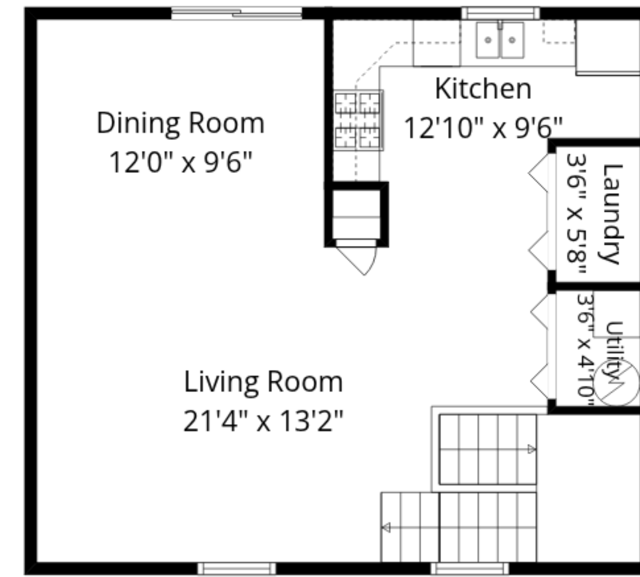
Upper Floor
